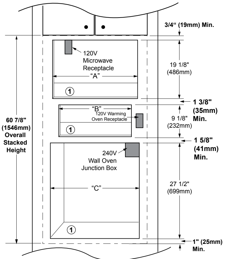
CUTOUT DIMENSIONS DCM24 SHOWN
