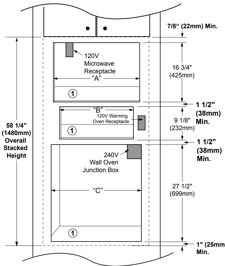
CUTOUT DIMENSIONS DMT2420 SHOWN
