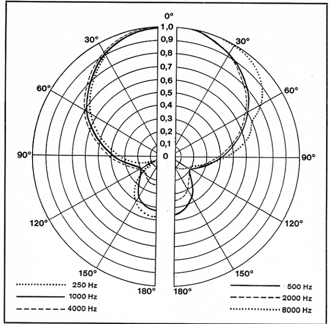
Polar diagram MD 415 N
