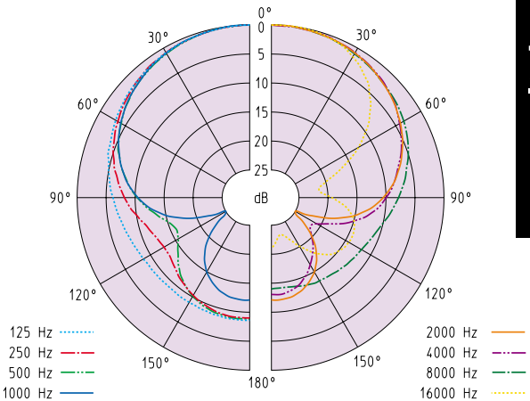
Polar Pattern
