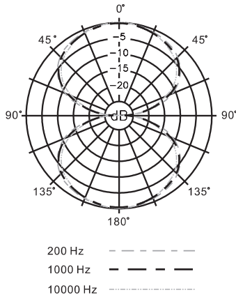
VR88 Polar Response
