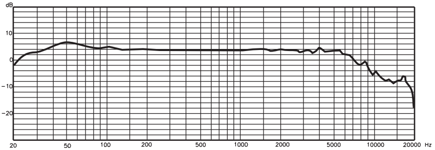
VR88 Frequency Response
