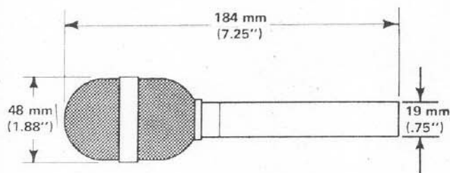
FIGURE 1 - Dimensions
