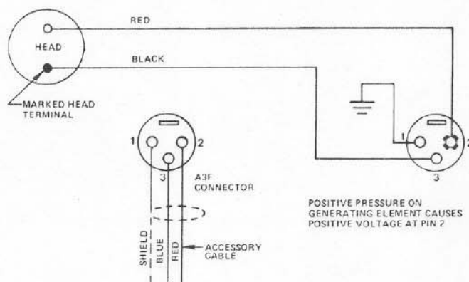
FIGURE 2 - Wiring Diagram
