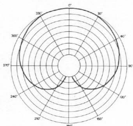
FIGURE 3 Polar Response
