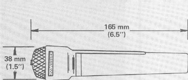
FIGURE 1 – Dimensions
