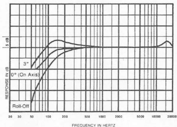
FIGURE 1 — Frequency Response
