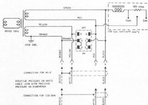
Figure 4 - Wiring Diagram
