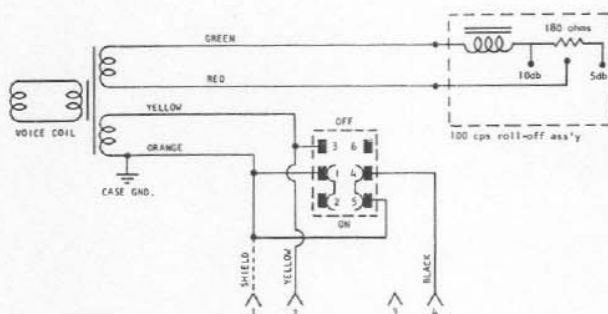
Figure 5 - Wiring Diagram, Modified
