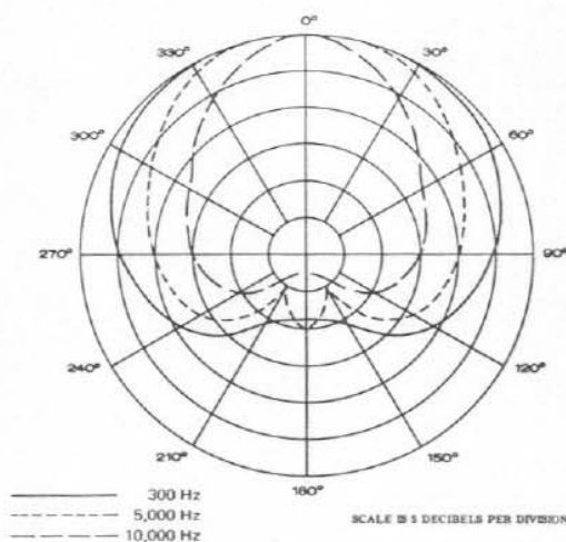
Figure 2 - Polar Pattern
