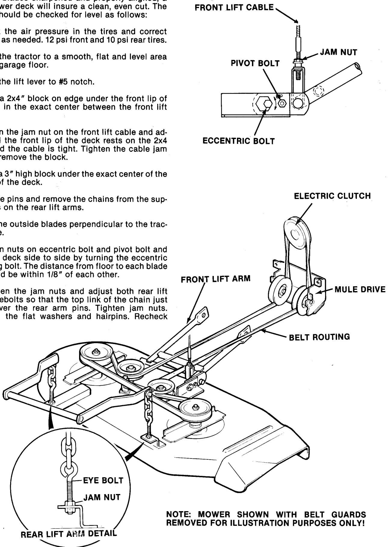
FIGURE 25 - 41" MOWER (TWO BLADE)
