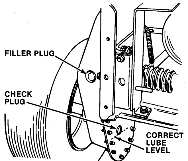
FIG. 12 - TRANSMISSION LUBE LEVEL
