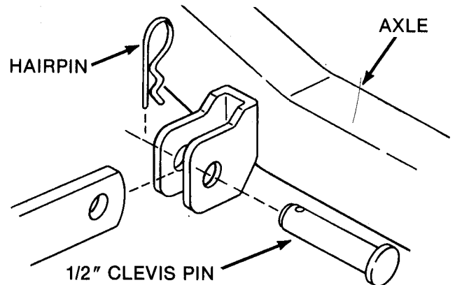
FIGURE 22 - FRONT LIFT ARM
