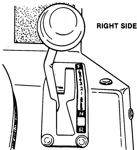
FIG. 5 - GROUND SPEED SELECTOR
