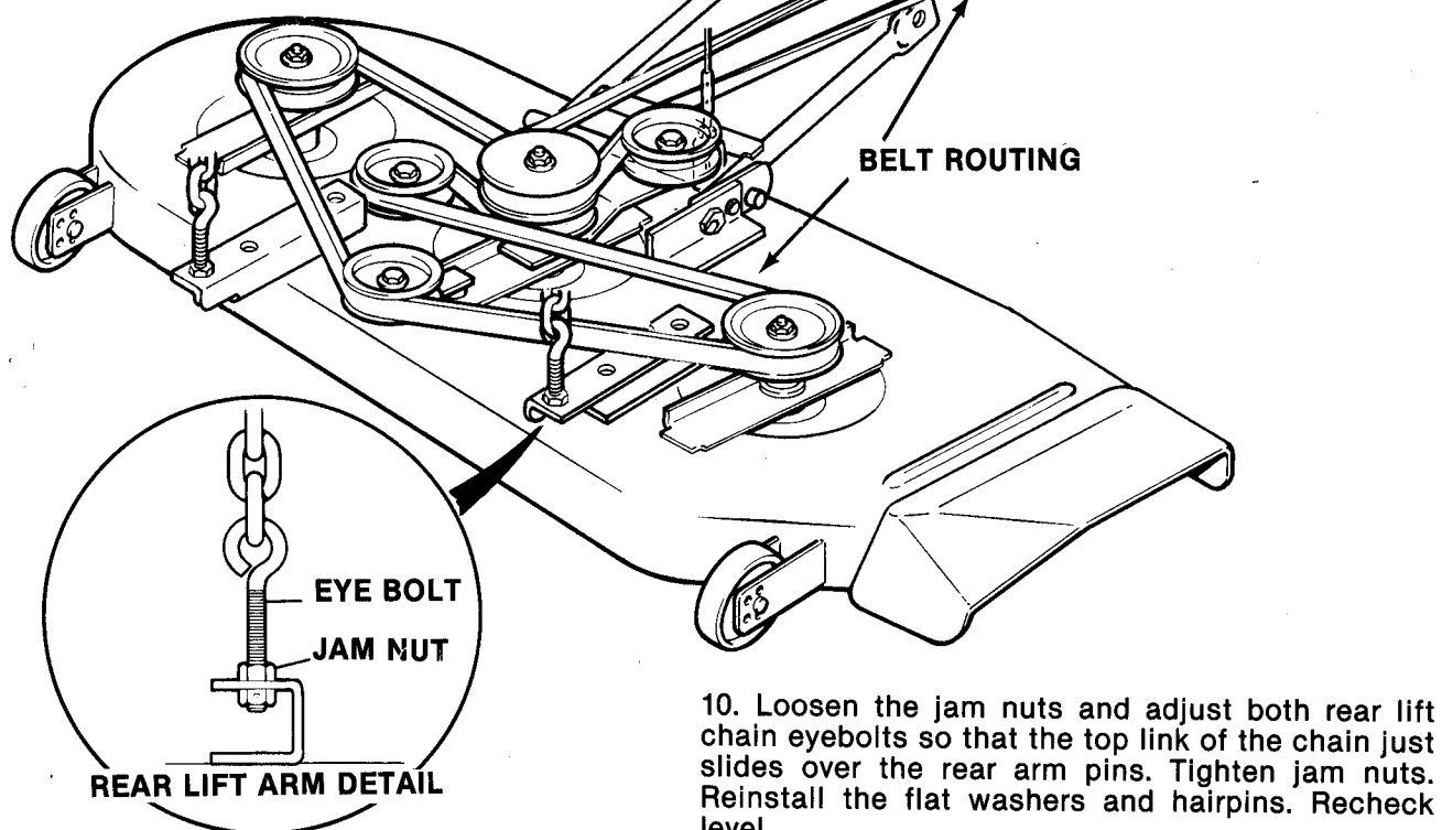
FIGURE 26 - 48" MOWER (3 BLADE)
