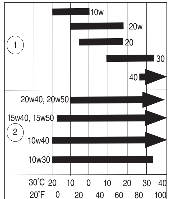
Figure 9-2 Ambient Temperature
