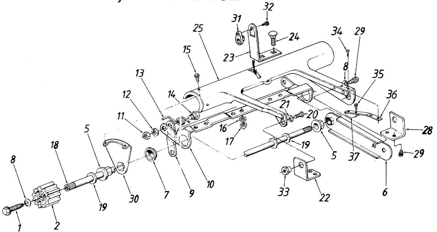
PARTS LIST FOR MODEL 280, 281 AND 282 ROTARY MOWERS
