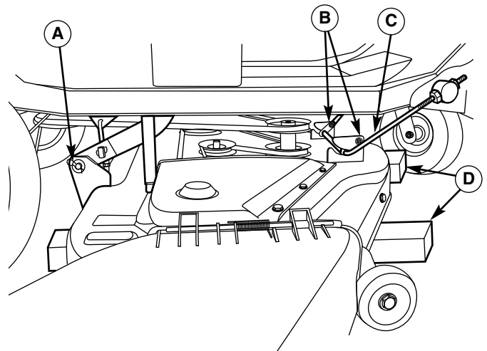
Figure 10. Mower Hitch Components A. Hair Pin Clip B. 3/8-16 x 3/4 Carriage Bolt & Flange Nut C. Hitch Rod D. 4x4 Wood Blocks
