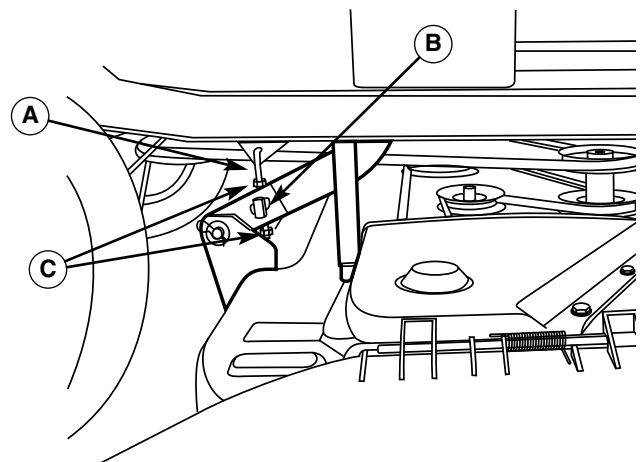
Figure 37. Side-to-Side Adjustment
