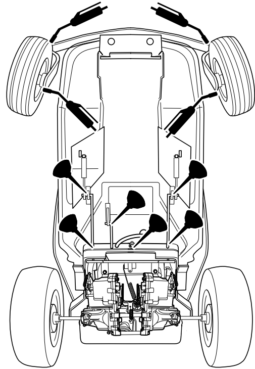
Figure 17. Lubricating Rider
