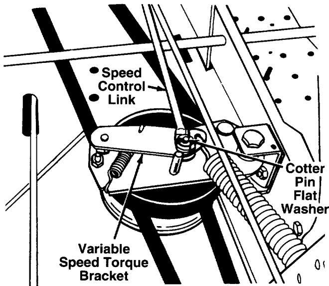
FIGURE 14.—Viewed From Beneath Tractor
