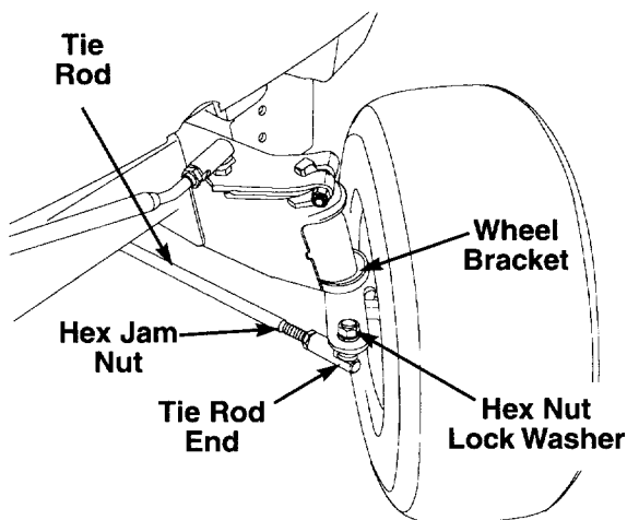
FIGURE 13.—Units with adjustable tie rods
