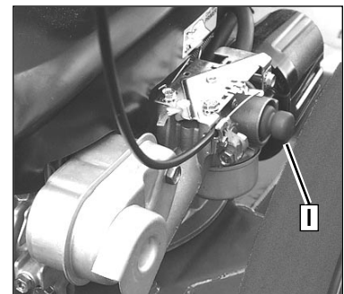
Figure 3-2: Engine primer.
