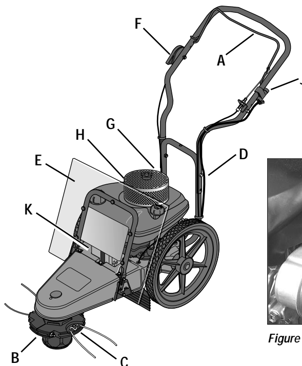
Figure 3-1: Features and controls (electric start model shown).
