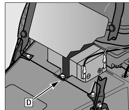
Figure 5-9: Battery replacement.
