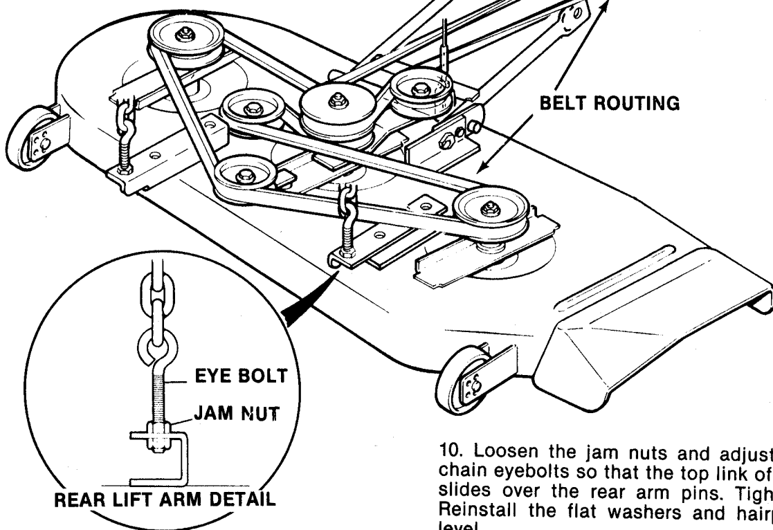
FIG. 31 - 48" MOWER LEVELING DETAIL
