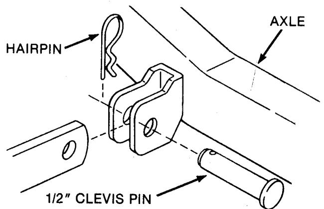
FIG. 27 - FRONT LIFT ARM DETAIL
