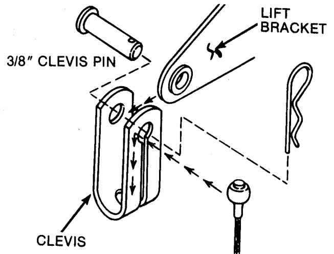
FIG. 26 - FRONT LIFT BRACKET
