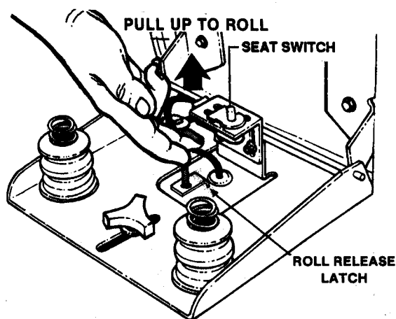
FIG. 7 - LATCH RELEASE UP TO ROLL
