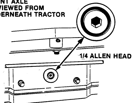
FIG. 15 - ENGINE OIL DRAIN LOCATION
