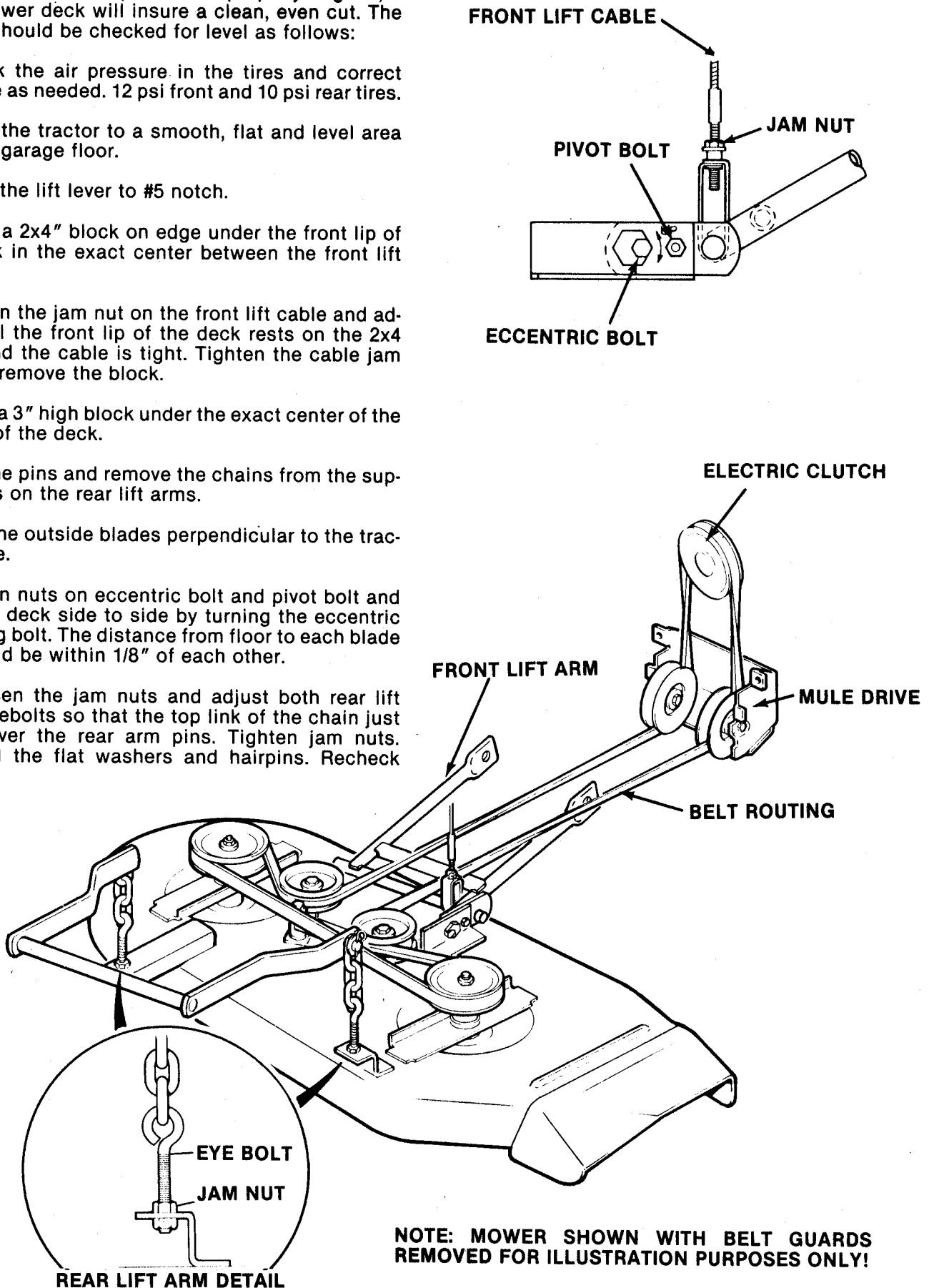
FIG. 30 - 41" MOWER LEVELING DETAIL
