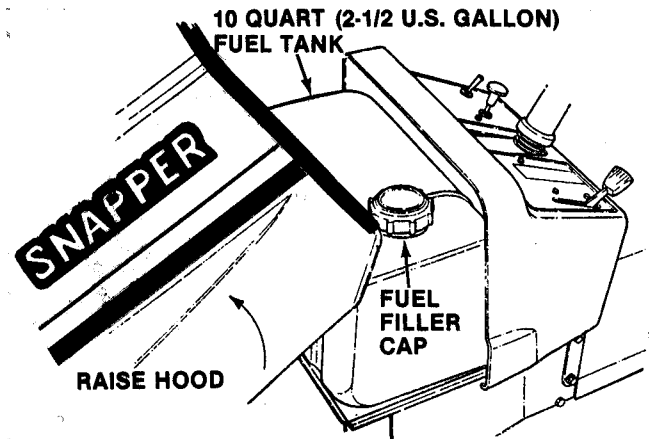
FIG. 3 - FUEL TANK UNDER HOOD
