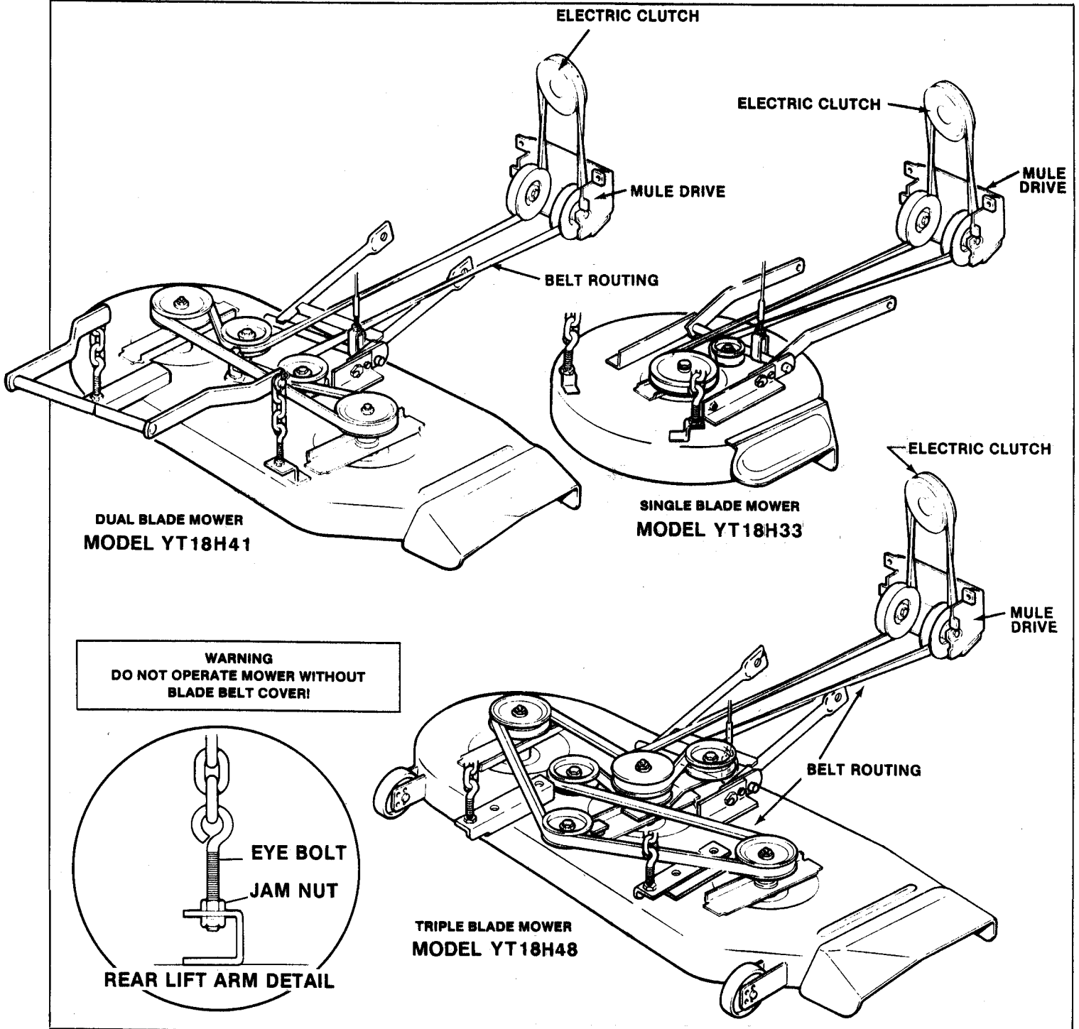
FIG. 24 · MOWER BELT ROUTING DETAIL
