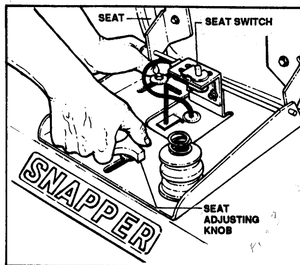
FIG. 8 - OPERATOR'S SEAT ADJUSTMENT
