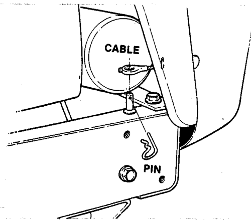
FIG. 11 - RELEASE CABLE TO TILT HOOD FULL FORWARD
