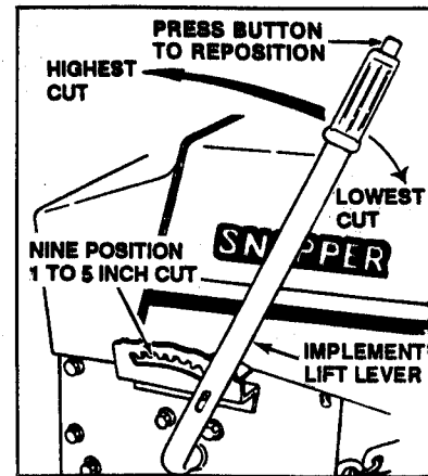
FIG. 10 - IMPLEMENT LIFT LEVER
