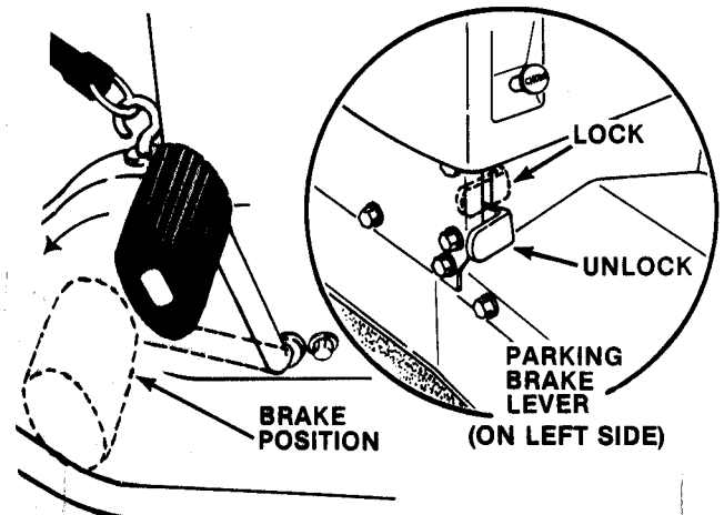
FIG. 4 - NEUTRAL RETURN/BRAKE PEDAL
