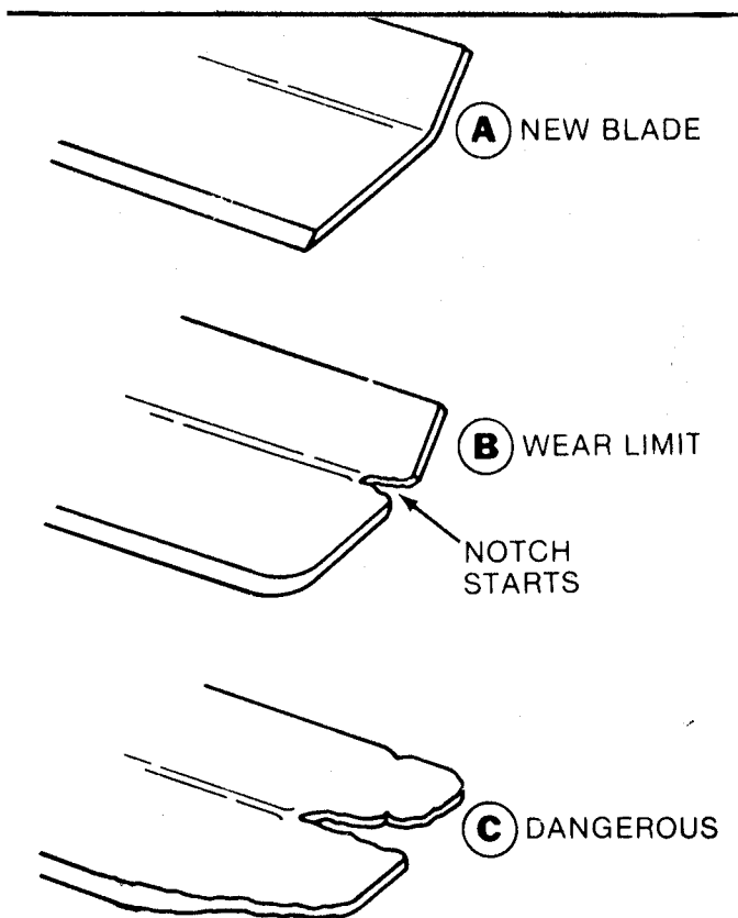
FIG. 21 - BLADE TIP WEAR PATTERNS
