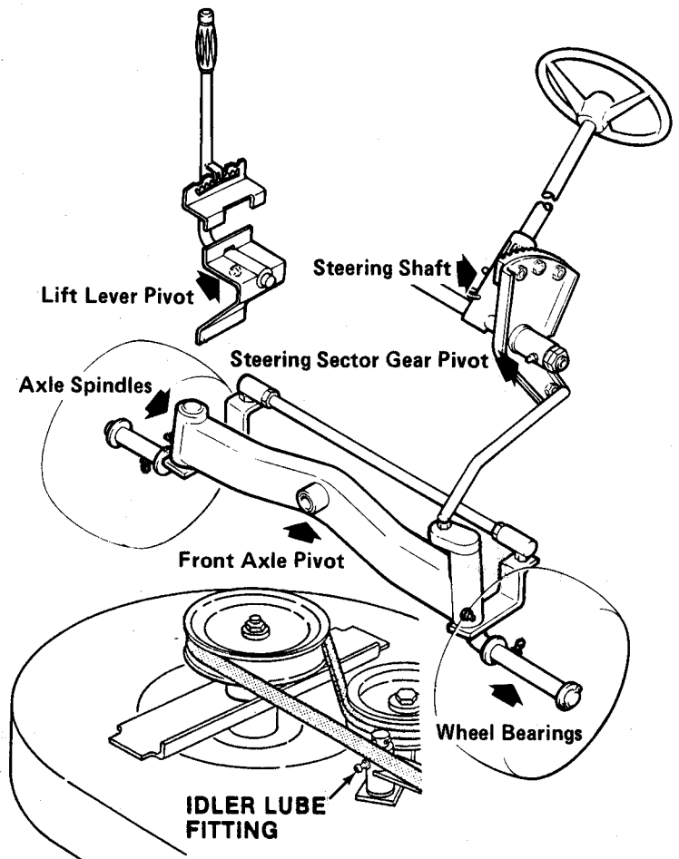
FIG. 14 - LUBRICATION POINT SCHEMATIC
