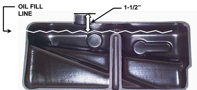
HYDRAULIC OIL RESERVOIR
