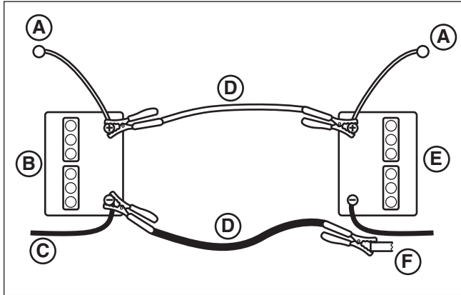
Figure 45. Jump Starting
