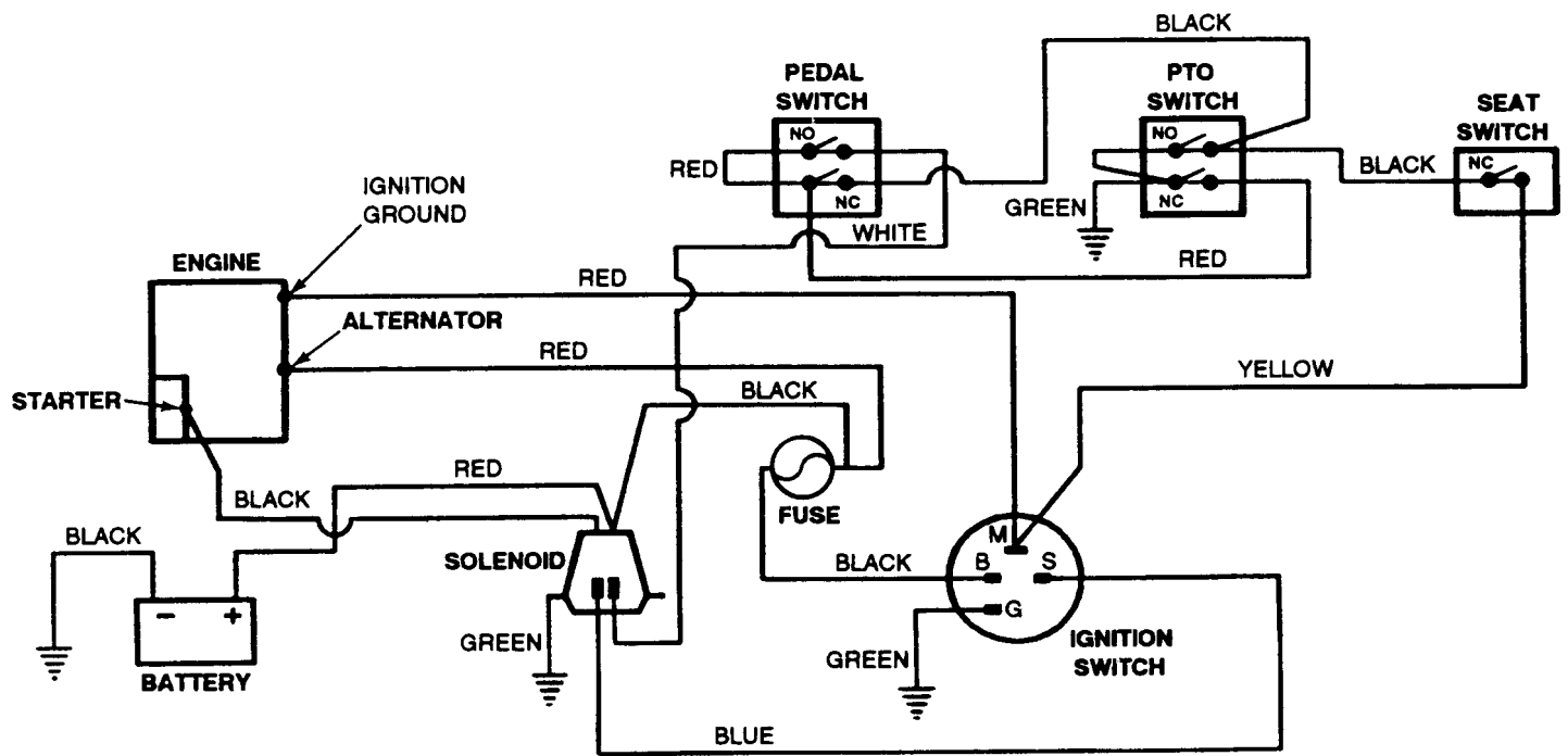
SCHEMATIC
