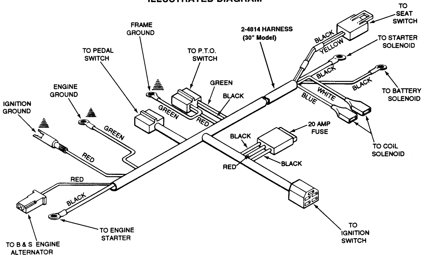
ILLUSTRATED DIAGRAM
