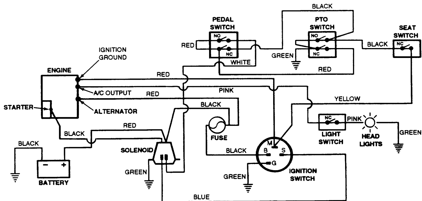
SCHEMATIC
