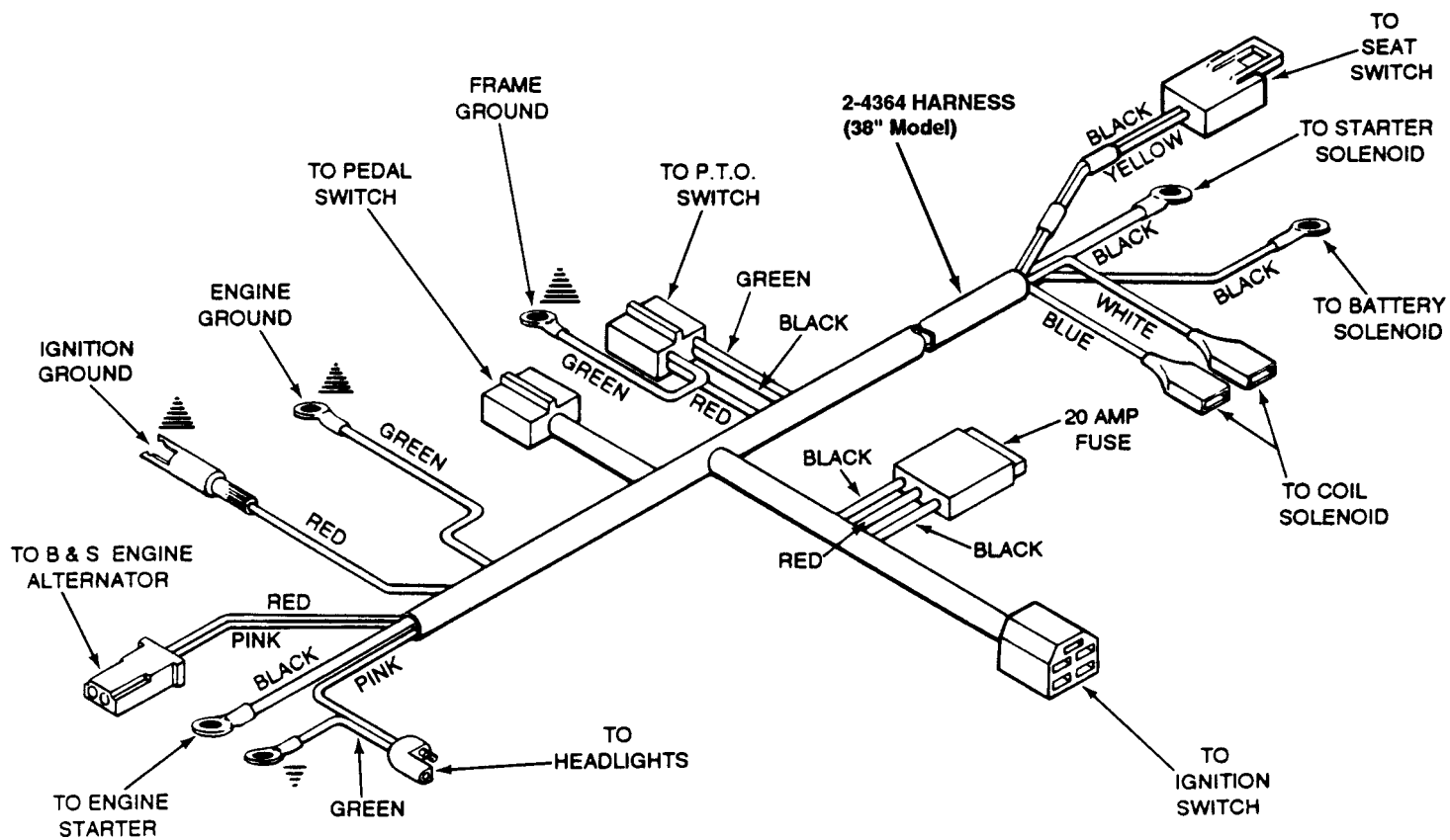
ILLUSTRATED DIAGRAM
