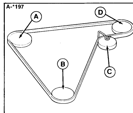
Figure 27. Belt Pattern, 36\" Mower
