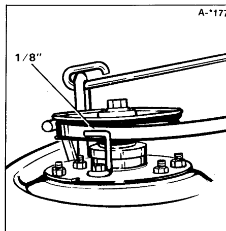
Figure 19. Left Mower Pulley Belt Stop
