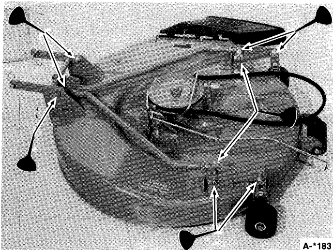
Figure 5. 26" & 30" Mower Lubrication Points
