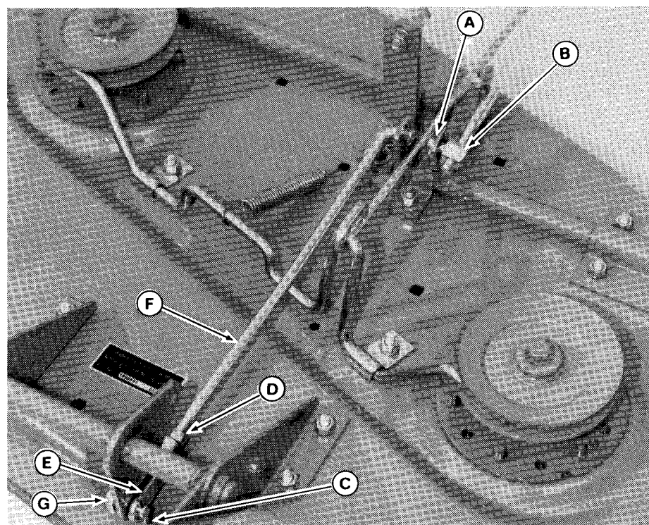
Figure 18. 36" Mower Leveling
