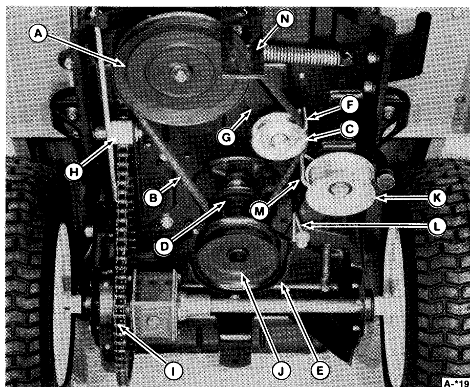
Figure 20. Rider & Mower Drive
