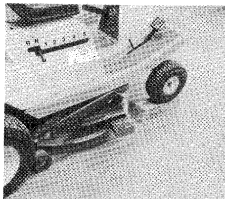
Figure 8. Blade Removal
