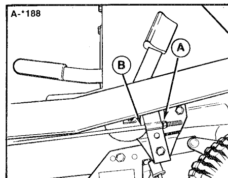
Figure 13. Clutch-Brake Adjustment A. Locknut B. Clutch-Brake Rod
