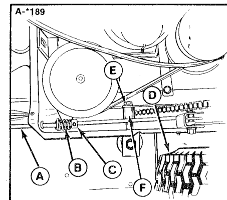
Figure 14. Clutch-Brake Adjustment (Viewed from underneath rider)
