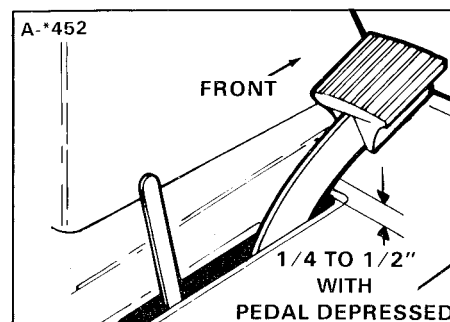
Figure 12. Clutch-Brake Adjustment
