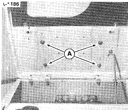
Figure 10. Seat Mounting Screws
