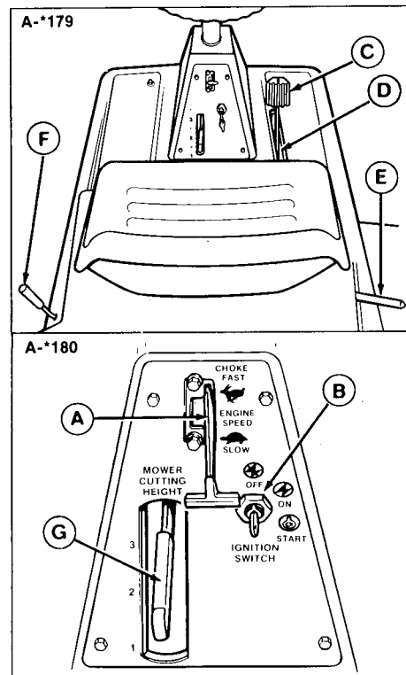
Figure 1. Rider & Mower Controls CHECKS BEFORE STARTING
