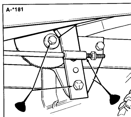
Figure 2. Clutch-Brake Pedal Lubrication (under right-hand footrest)
