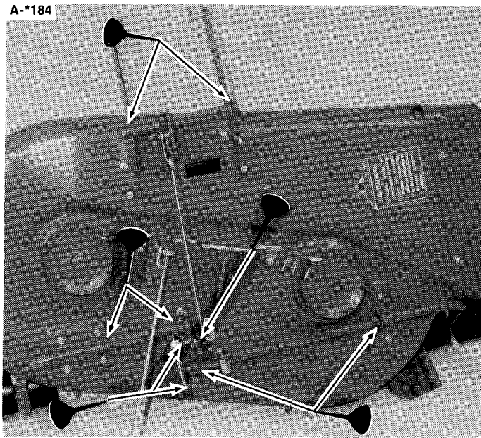
Figure 6. 36" Mower Lubrication Points
