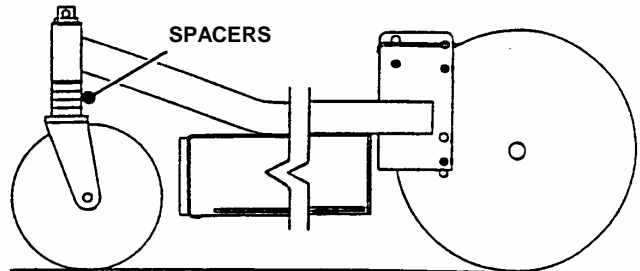
FIGURE 3.14D: HIGH CUT 3-3/4" TO 4-3/4"
