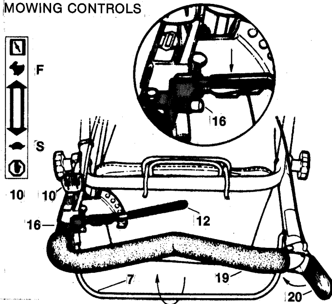
FIG. 6 MOWING CONTROLS
