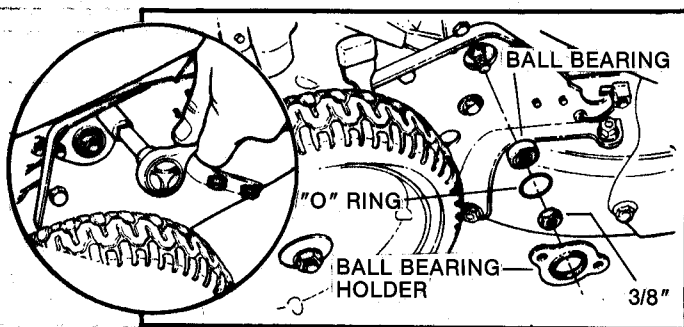
FIG. 16-A BEARING REPLACEMENT
