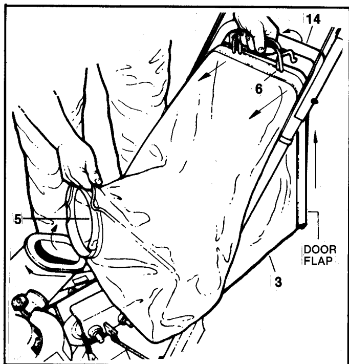
FIG. 7-EMPTYING GRASS BAG
