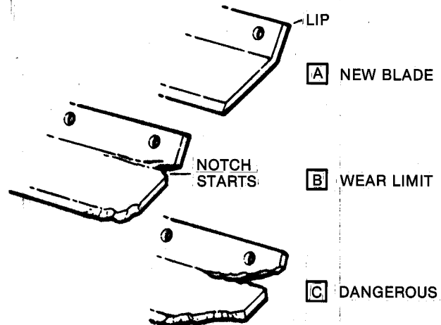
FIG. 9-BLADE WEAR PATTERNS
