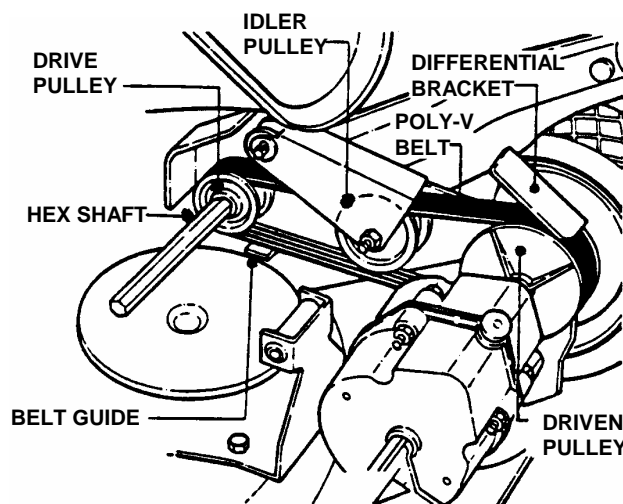
ROUTING OF POLY-V-BELT
