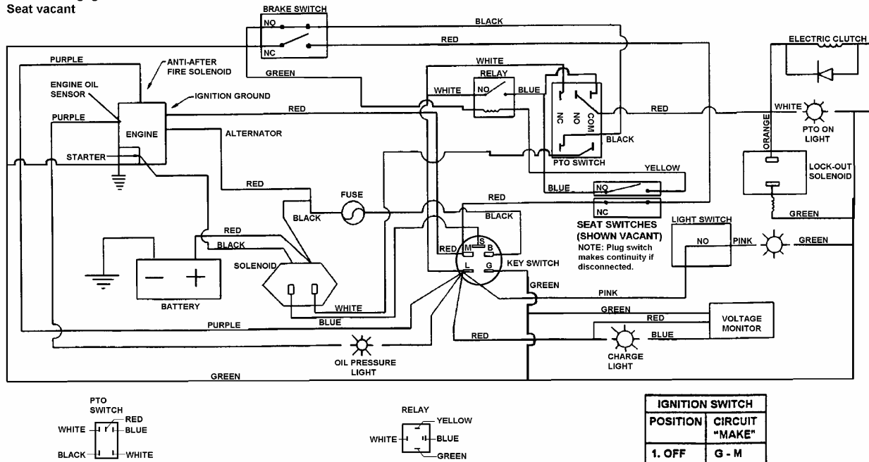
LT180H42IBV2 & LT200H48IBV2 SCHEMATIC - WIRING HARNESS P/N 73417
