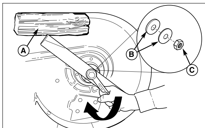
Figure 20. Blade Installation Mowers (38" & 40" Mowers) A. 4x4 Wood Block B. Spring Washers C. Blade Nut
