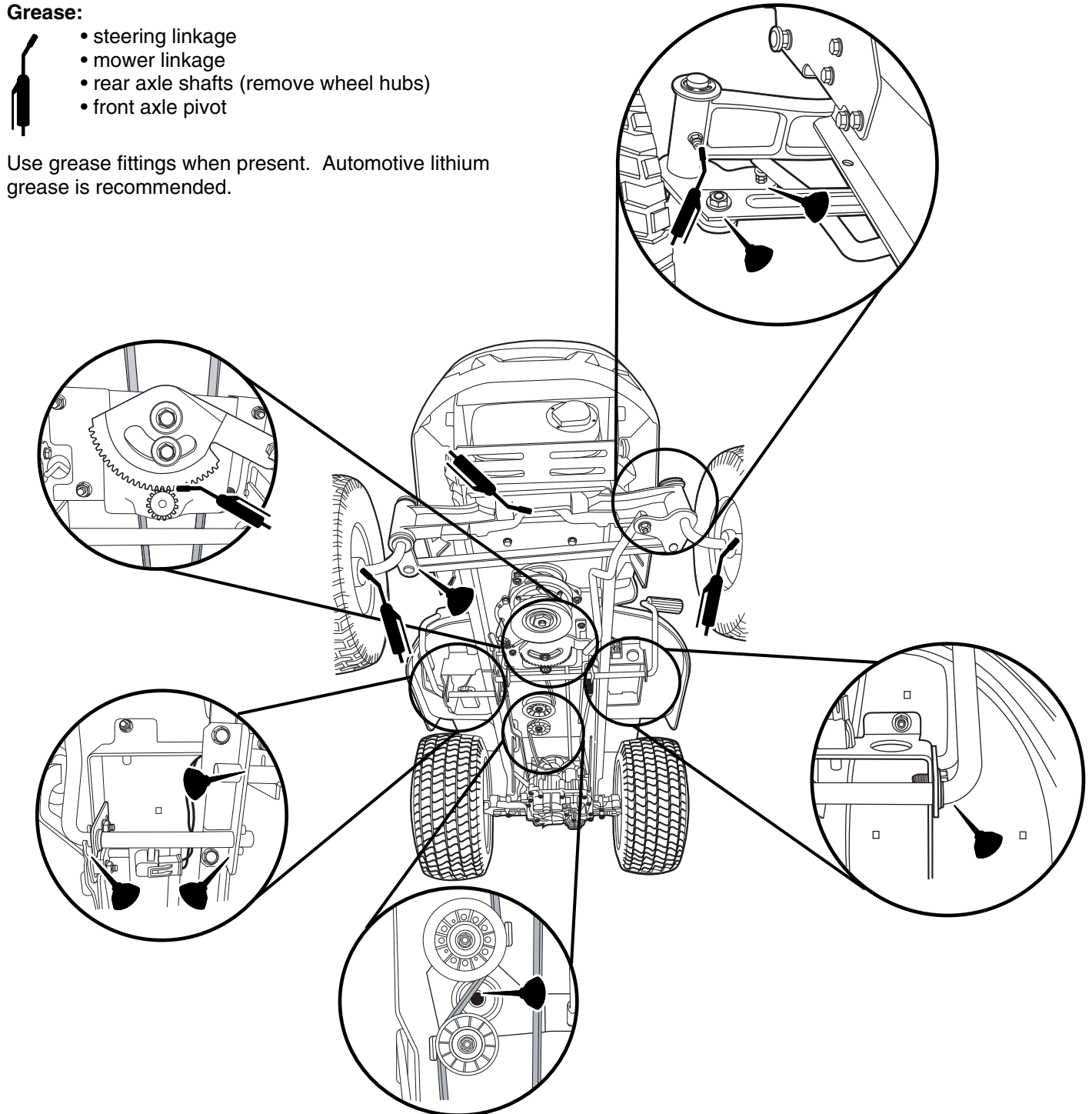
Figure 14. Lubricate Tractor
