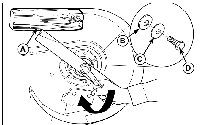
Figure 21. Blade Installation Mowers (44" Mowers) A. 4x4 Wood Block B. Hex Washer C. Spring Washer D. Blade Capscrew
