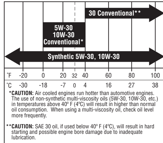
Figure 25. Recommended Engine Oil - Briggs & Stratton Models
