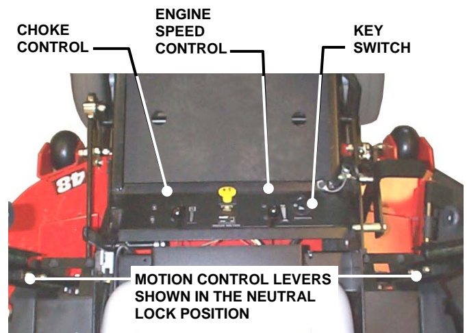
SHOWN FROM OPERATOR'S VIEW POINT
