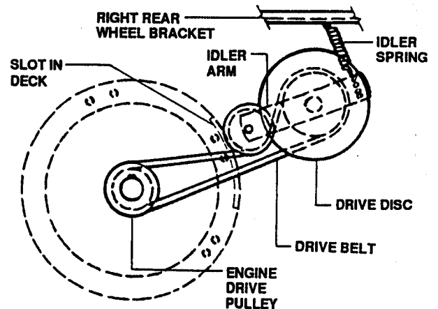
TOP VIEW OF ENGINE BELT ROUTING
