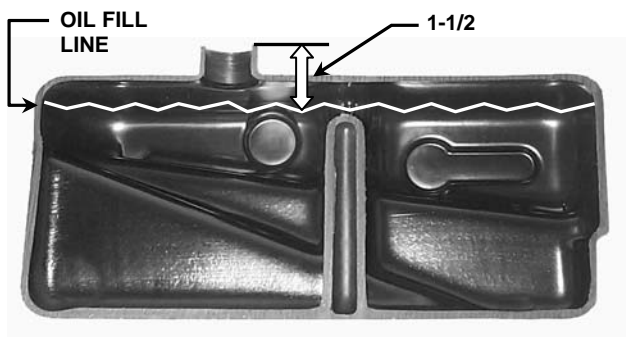
HYDRAULIC OIL RESERVOIR
