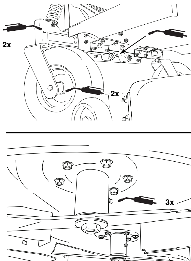
Figure 13. Lubrication Points (Grease)
