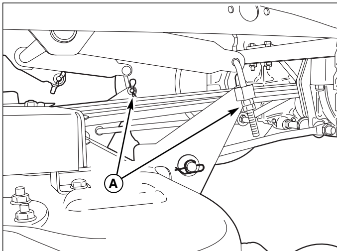
Figure 29. Mower Leveling - Side-to-Side A. Rear Leveling Nuts (Left side shown, right side hidden)
