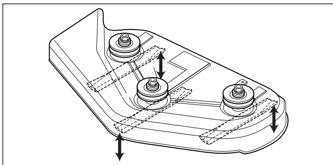
Figure 30. Orient Blades Front-to-Back
