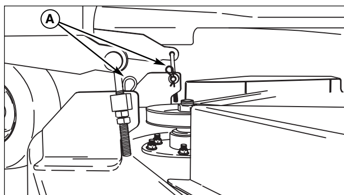
Figure 12. Front Deck Lift Components A. Hairpin Clip & Washer (Left & right)
