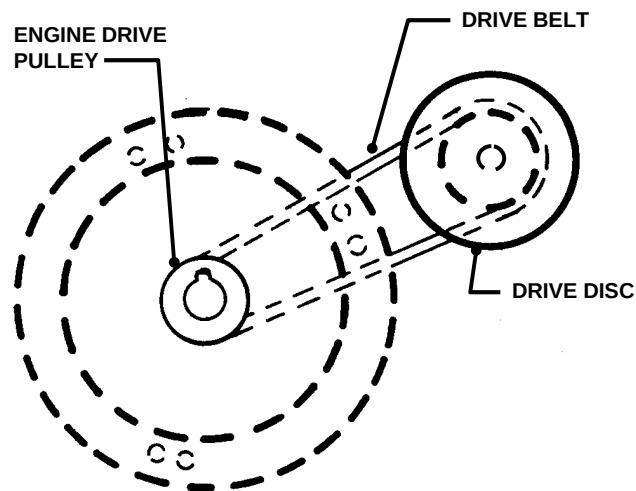
TOP VIEW OF STRETCH TYPE BELT ROUTING
