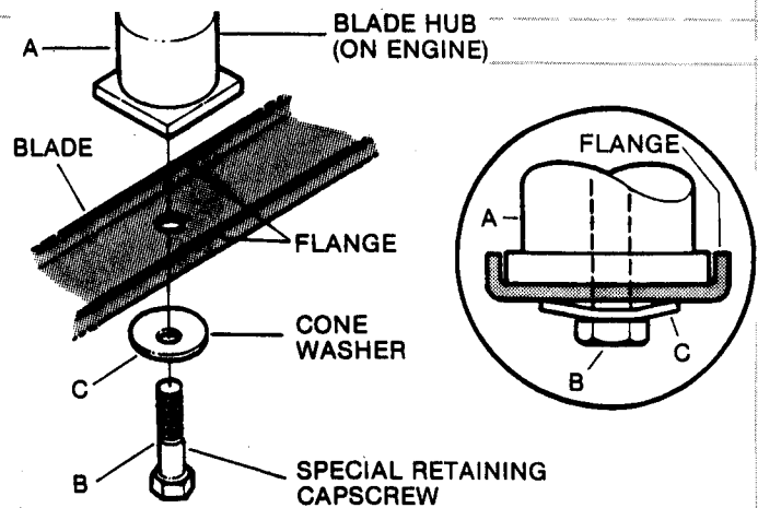
FIG. 10 - BLADE RETENTION DETAIL
