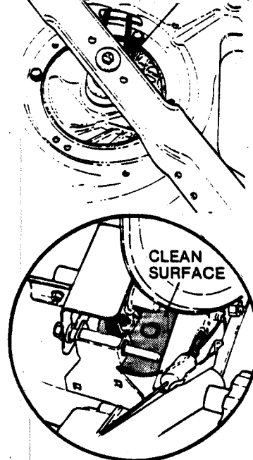
OIL PLUG-DRAIN (UNDER DECK)
