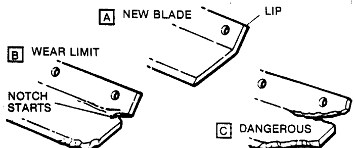
FIG. 9-BLADE WEAR PATTERNS
