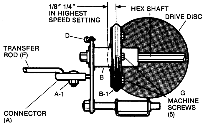
FIG. 13 -DRIVEN DISC COMPONENTS
