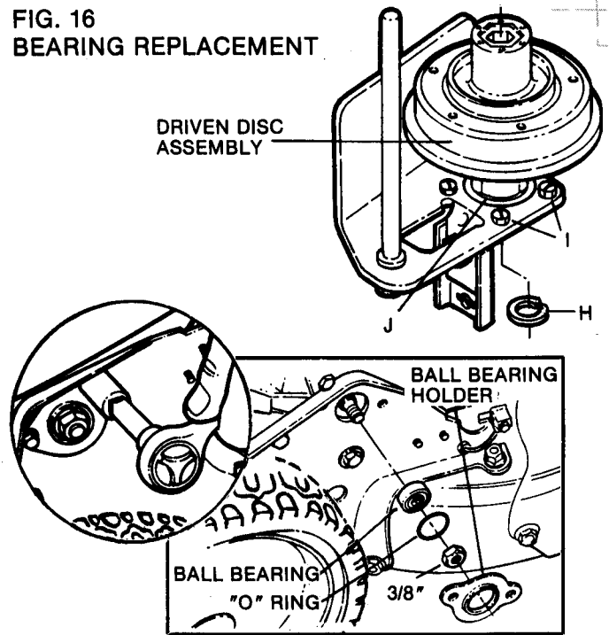
FIG. 16-A - BEARING REPLACEMENT
