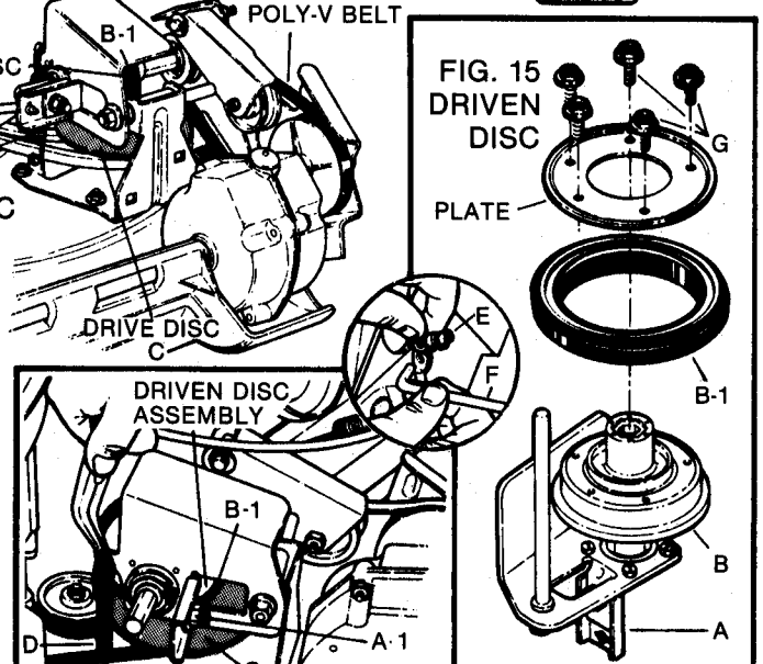
FIG. 14 DRIVEN DISC ASSEMBLY
