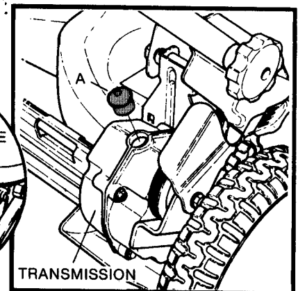
FIG. 7 TRANSMISSION PLUG A
