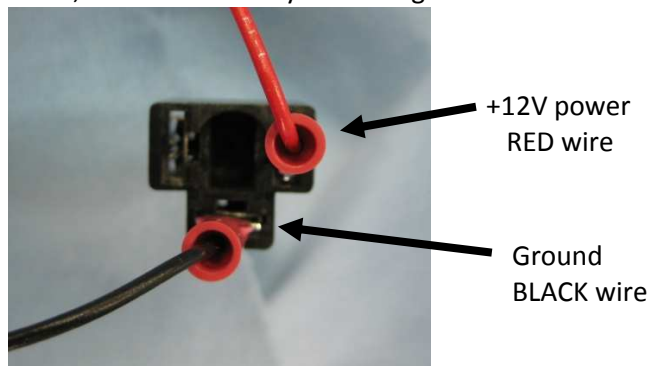
Original plug with jumper wires for power and ground connected
