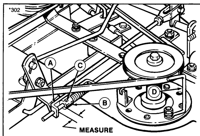
Figure 34. Drive Belt Tension
