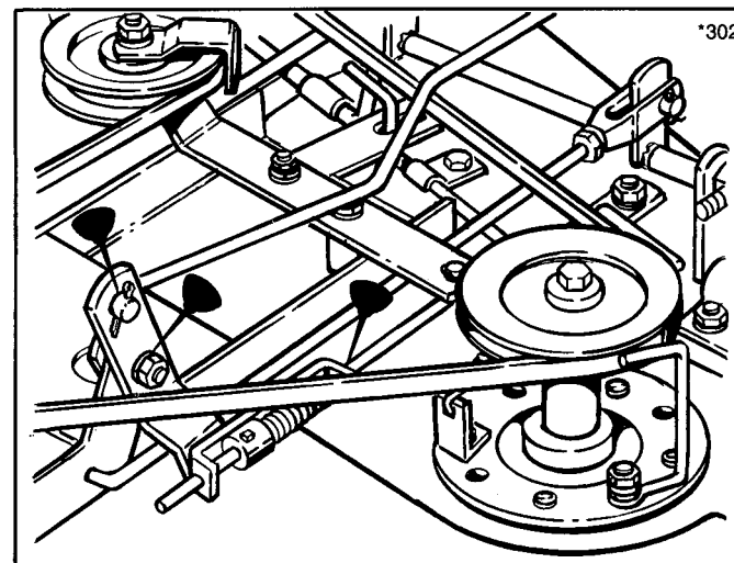
Figure 18. Lubricate Height, PTO Rod and PTO Arm.
