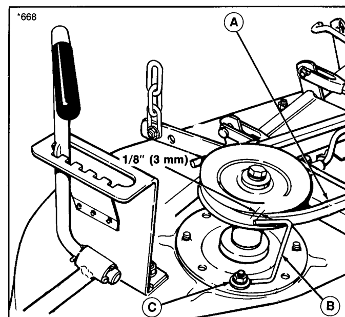
Figure 35. Right Arbor Belt Stop
