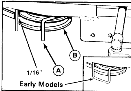
Figure 35. Right Hand Belt Stop, PTO Pulley - 42" Mower A. Belt Stop B. Drive Belt
