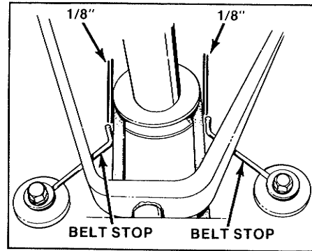
Figure 33. Drive Pulley Belt Stops TRACTOR ADJUSTMENTS - Serial No. 2535 and lower.
