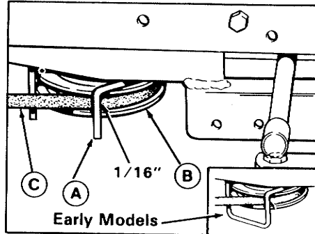
Figure 36. Right Hand Belt Stop, PTO Pulley - 36" Mower A. Belt Stop C. Belt B. PTO Pulley
