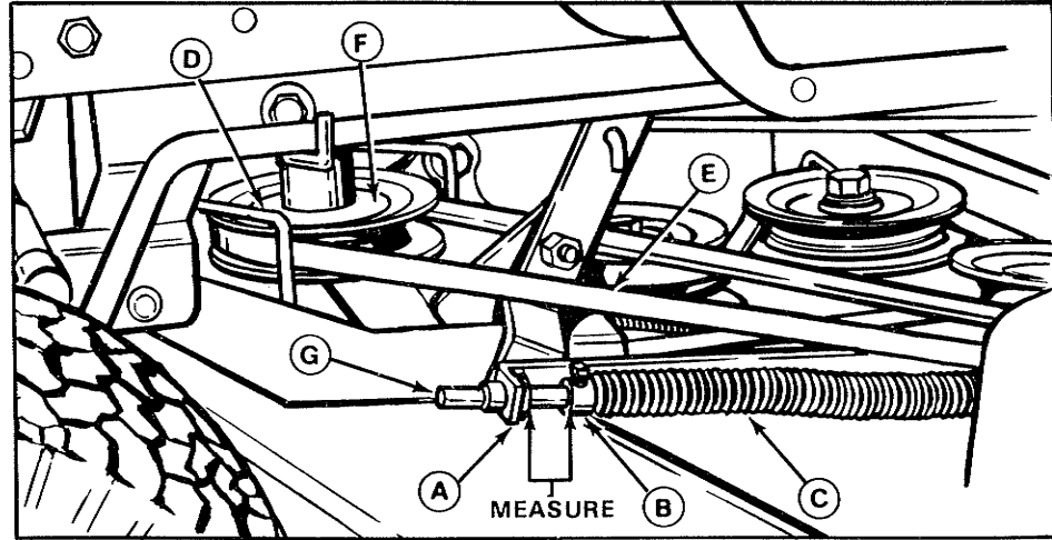
Figure 34. Mower Drive Belt Tension Adjustment - 42" Mower Shown.
