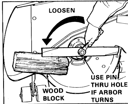
Figure 20. Removing Blade
