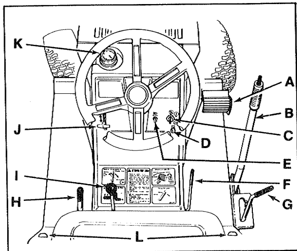
Figure 8. Tractor & Mower Controls
