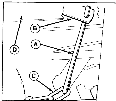
Figure 2. Installing Lift Link (Seen from right-hand side)
