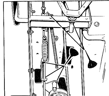
Figure 12. Clutch & Brake Rod Lubrication
