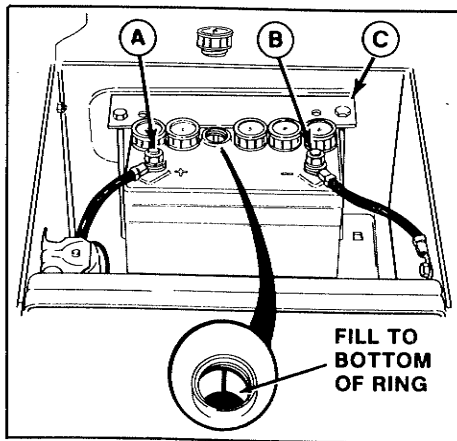
Figure 13. Battery
