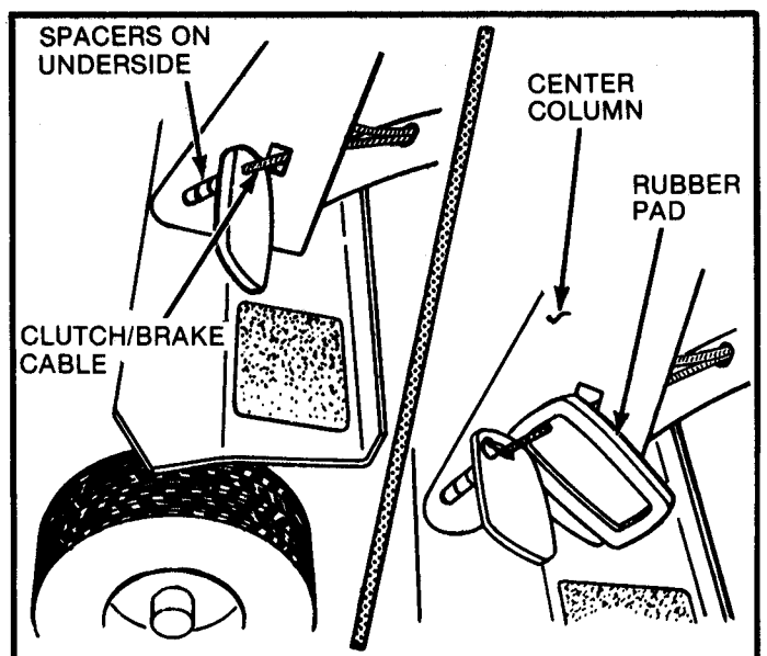
FIG. 10 — CLUTCH/BRAKE ADJUSTMENT
