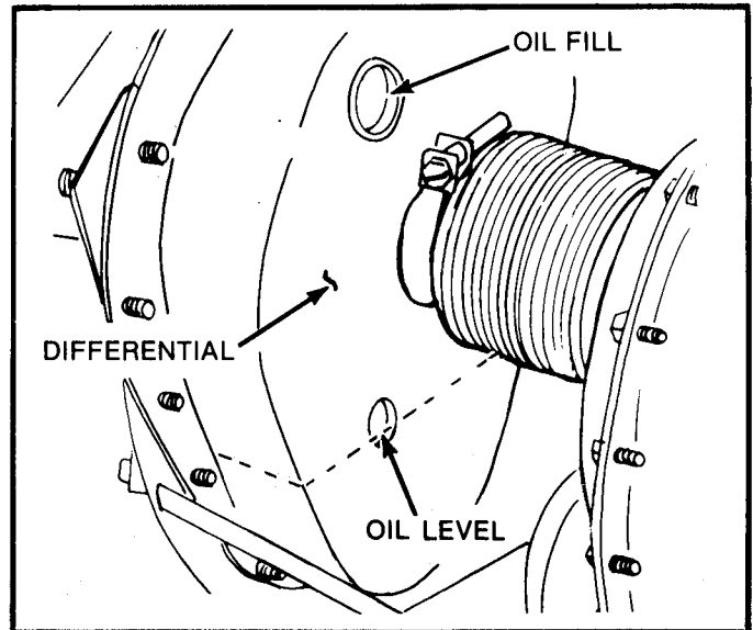
FIG. 3 — DIFFERENTIAL LUBE LEVEL
