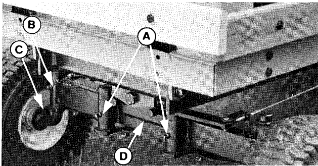
Figure 7. Grease Fittings
