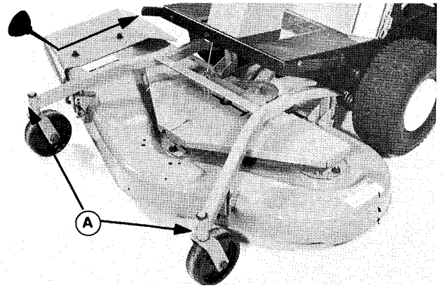
Figure 8. Grease Fittings & Lift Lever Pivot Points in Frame
