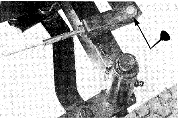
Figure 5. Lube Rear Axle Clevis and Pivot Points
