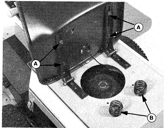
Figure 17. Seat Adjustment
