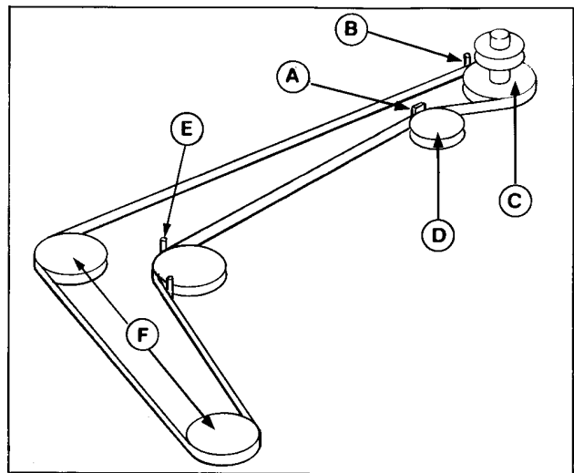
Figure 11B. 36" Mower Belt Pattern
