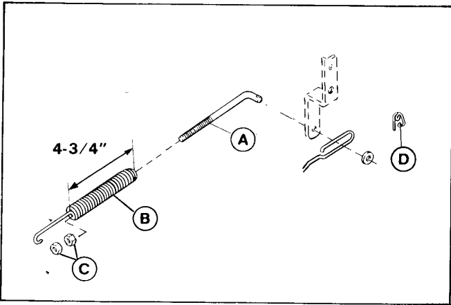
Figure 22. PTO, 42" Mower
