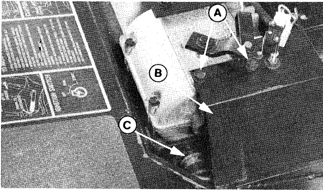
Figure 19. Chain Adjustment
