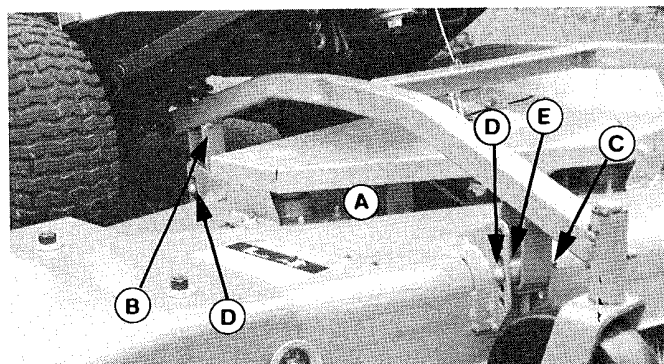
Figure 18. Mower Leveling
