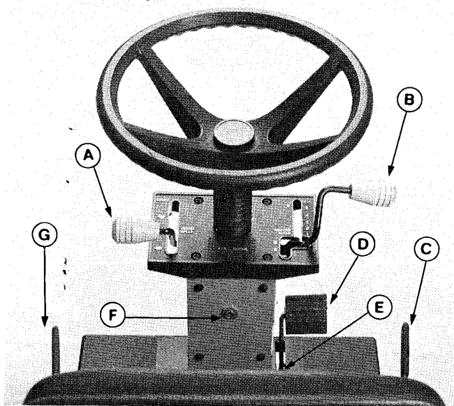
Figure 1. Controls
