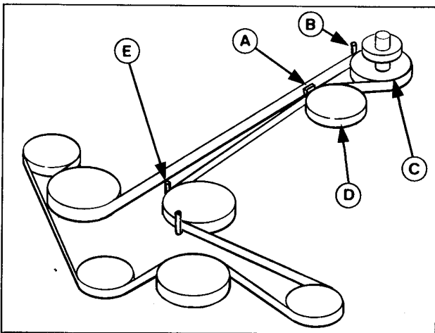
Figure 11A. 42" Mower Belt Pattern
