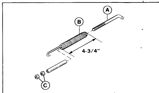
Figure 21. PTO, 36" Mower
