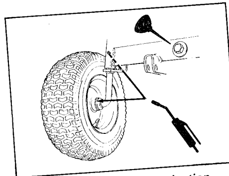
Figure 11. Front Axle Lubrication (Two grease fittings on each side)
