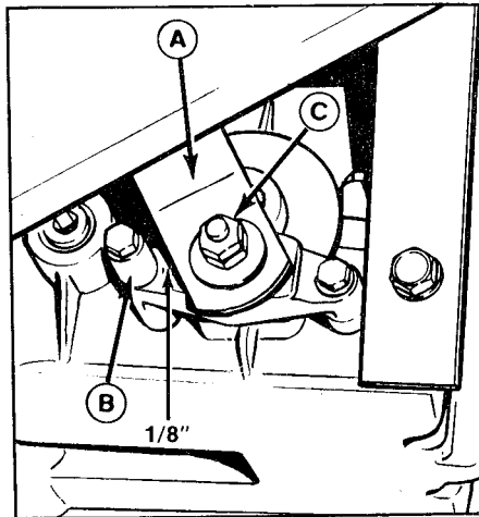
A. Brake Cam Lever B. Stop C. Adjustment Nut
