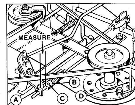
Figure 27. Drive Pulley Belt Stops
