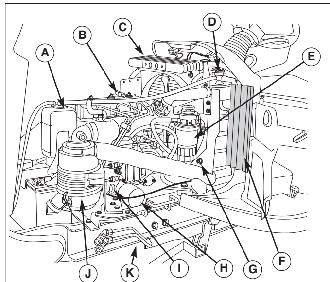
Figure 24. Engine
