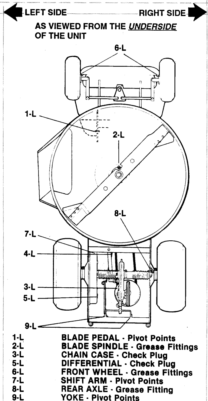
FIG. 2 - LUBRICATION & SERVICE POINTS
