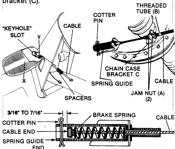
FIG. 12 - CLUTCH/BRAKE ADJUSTMENT
