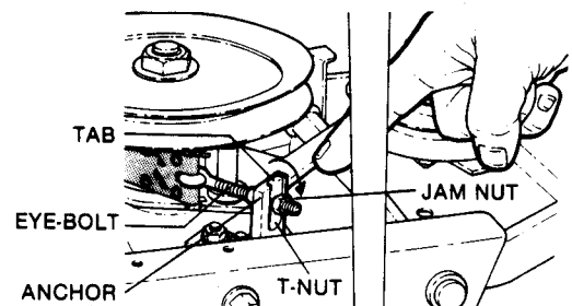
FIG. 11 - BLADE BRAKE ADJUSTMENT
