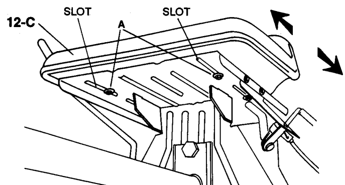
FIG. 7 - CHECK SEAT RETAINER SCREWS
