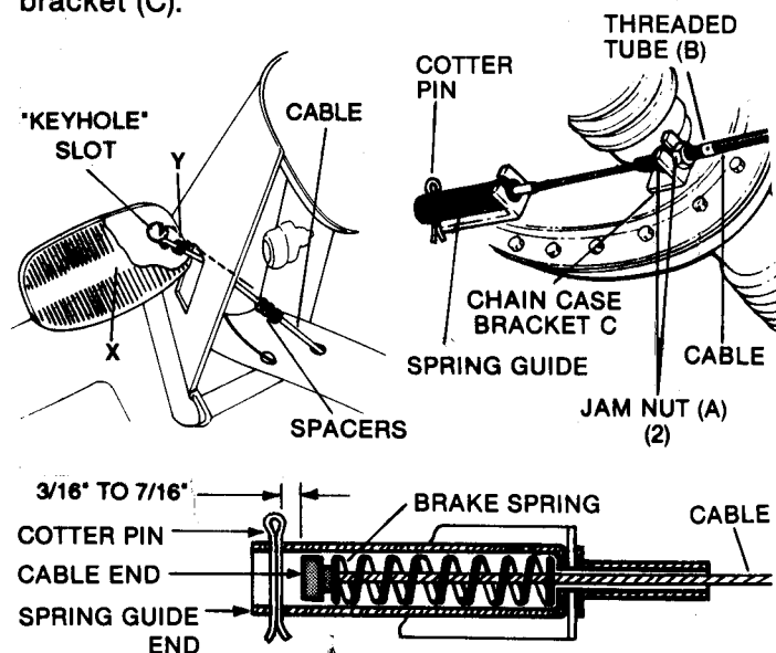
FIG. 12 - CLUTCH/BRAKE ADJUSTMENT
