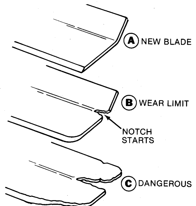
FIG 6 - BLADE WEAR PATTERNS
