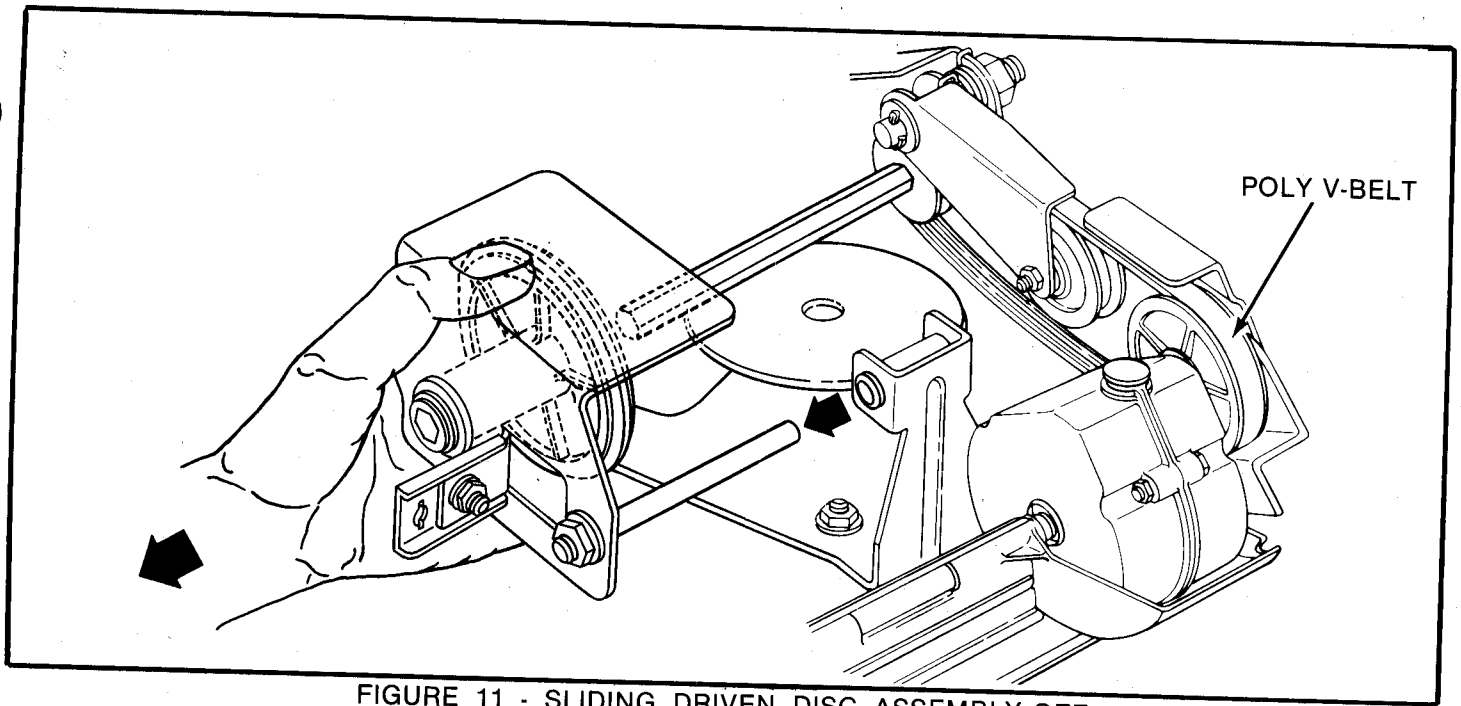
FIGURE 11 - SLIDING DRIVEN DISC ASSEMBLY OFF
