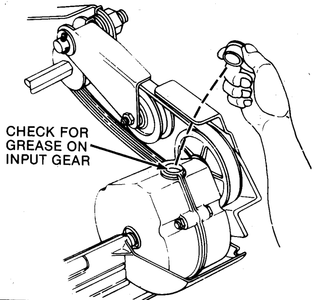
FIG. 5 - CHECKING TRANSMISSION
