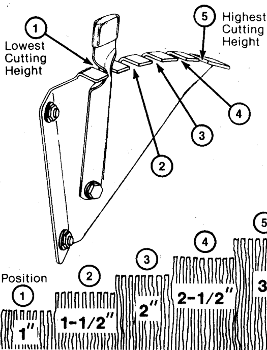
FIG. 3 - CUTTING HEIGHT SETTINGS
