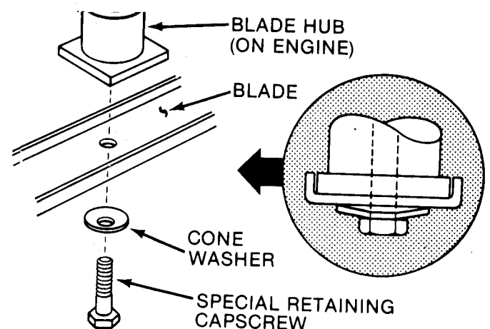
FIG 7 - BLADE RETENTION DETAIL
