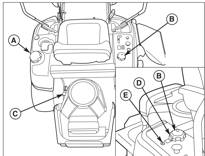
Figure 18. Maintenance A. Fuel Tank Cap B. Transmission Oil Cap C. Fuel Filter D. Locking Tab E. Locking Screw
