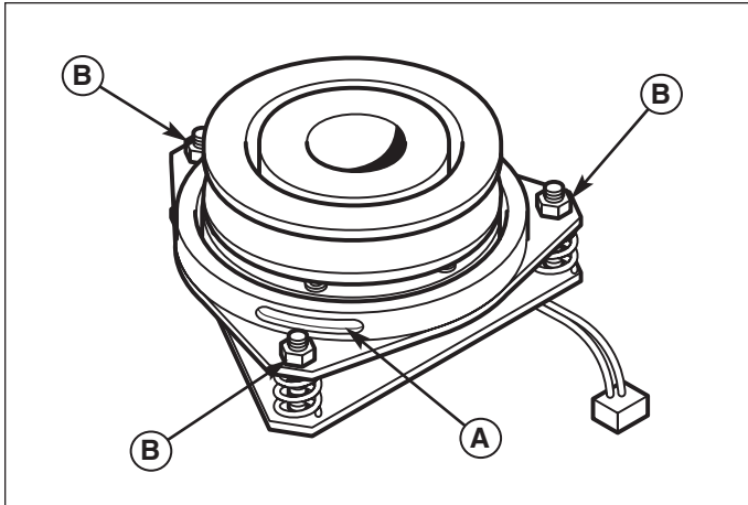
Figure 26. PTO Clutch Adjustment A. Adjustment Window (Qty. 3, one shown) B. Adjustment Nut
