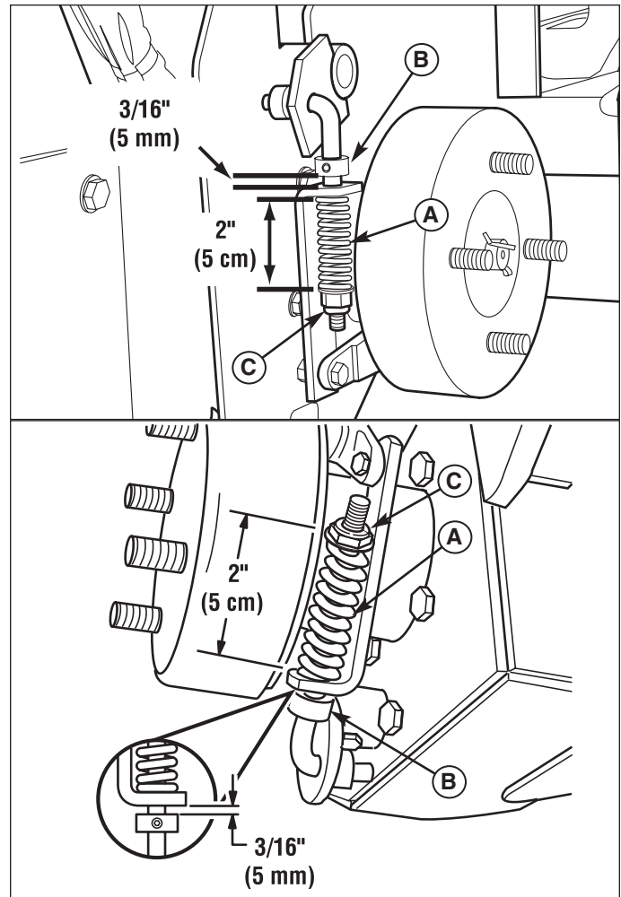
Figure 24. Parking Brake Adjustment
