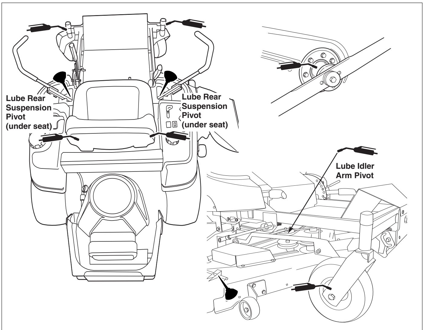
Figure 13. Lubrication
