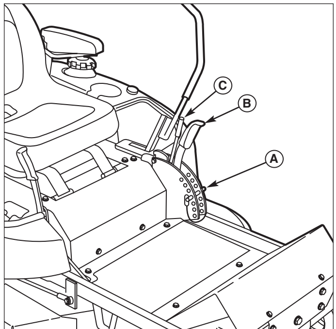
Figure 23. Cutting Height Adjustment A. Cutting Height Adjustment Pin B. Deck Lift / Cutting Height Lever C. Transport Release Lever
