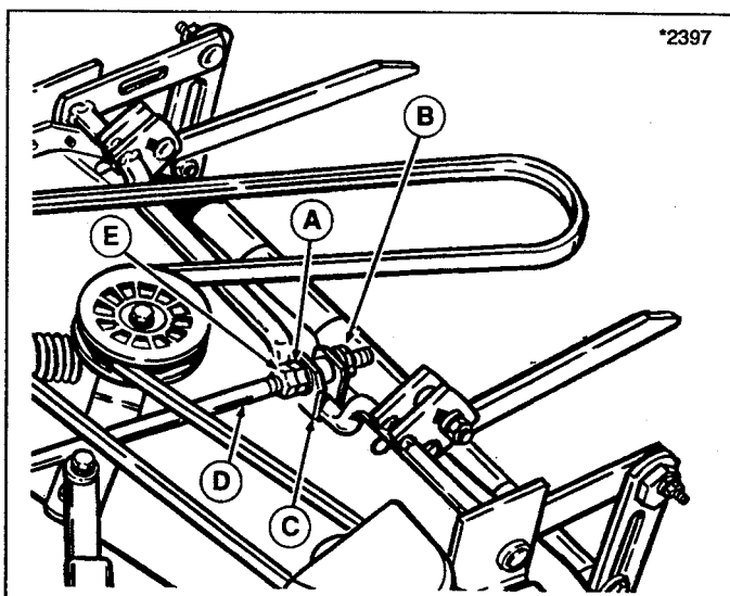
Figure 33. Front-To-Back Levelling
