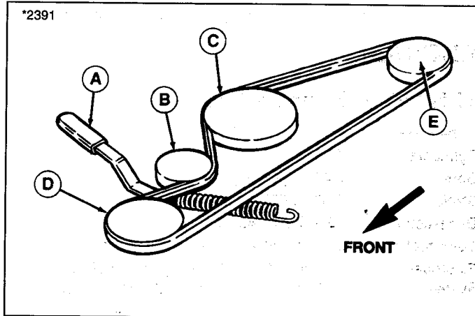
Figure 35. Belt Pattern - 30" Mower
