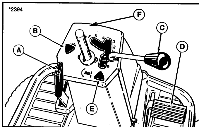
Figure 32. Dash Controls (shown with steering wheel removed)
