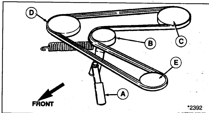
Figure 37. Belt Pattern - 34" Mower
