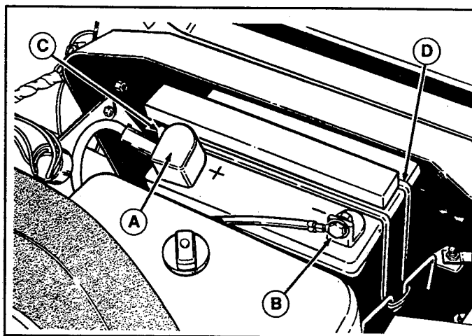
Figure 19. Battery
