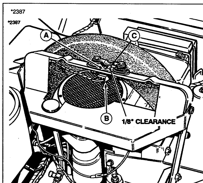
Figure 4. Seat Switch
