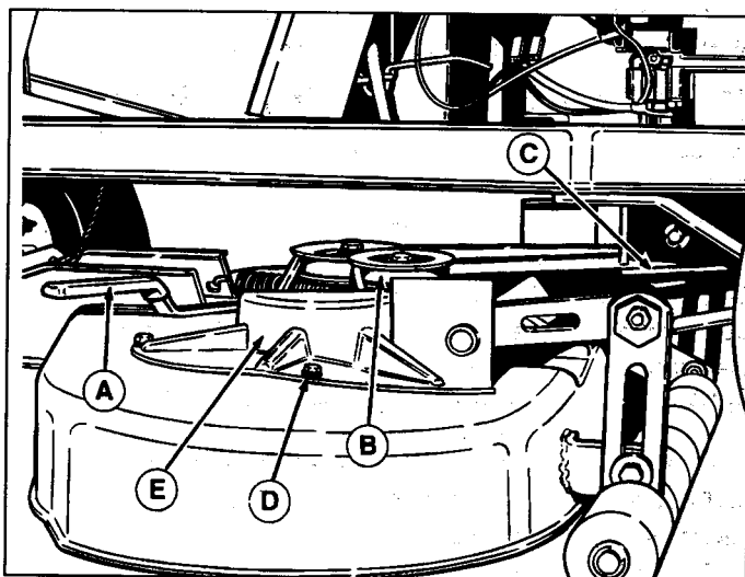
Figure 36. Mower Belt Replacement - 34"
