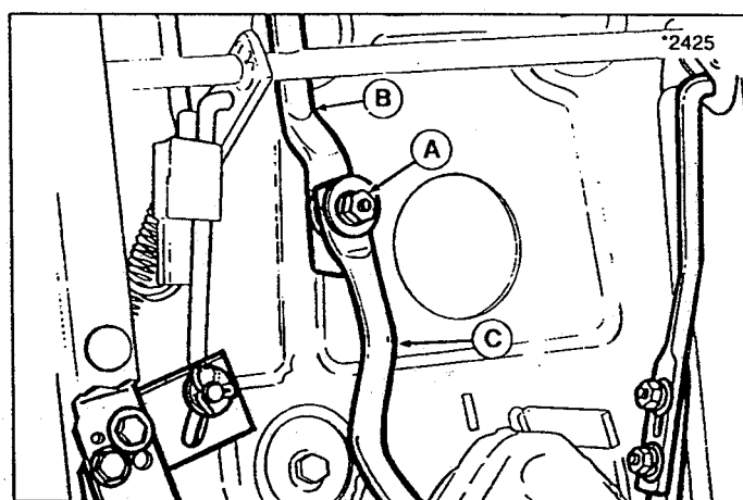
Figure 27. Neutral Adjustment - Hydro Models
