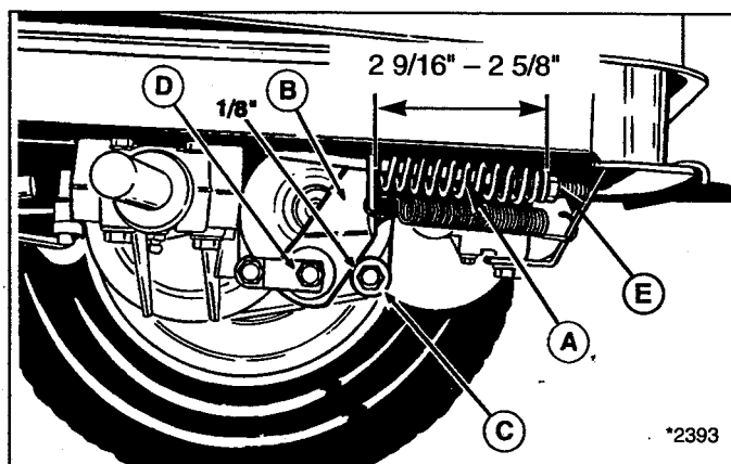
Figure 24. Brake Adjustment (Gear model)
