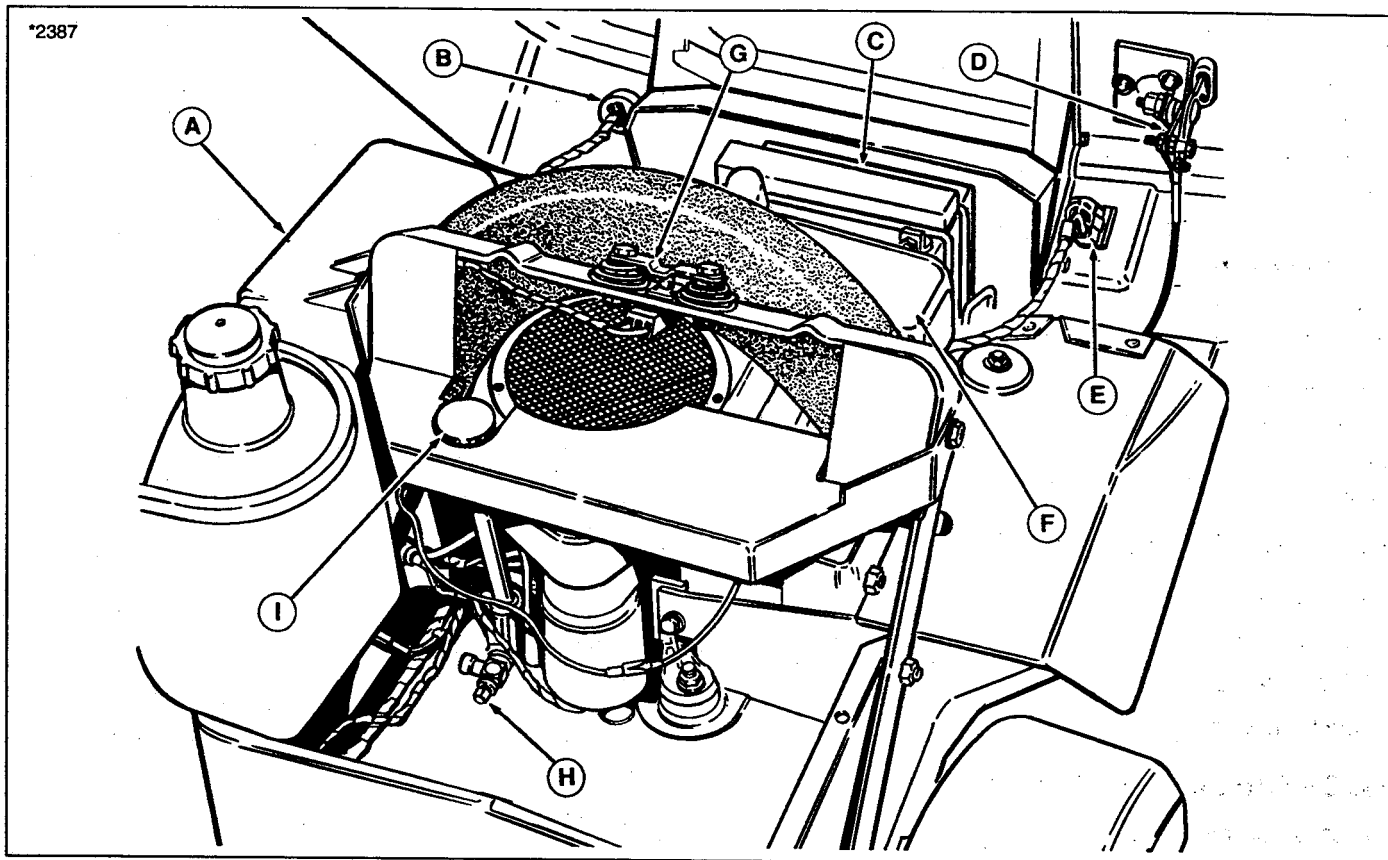
Figure 3. Engine Compartment
