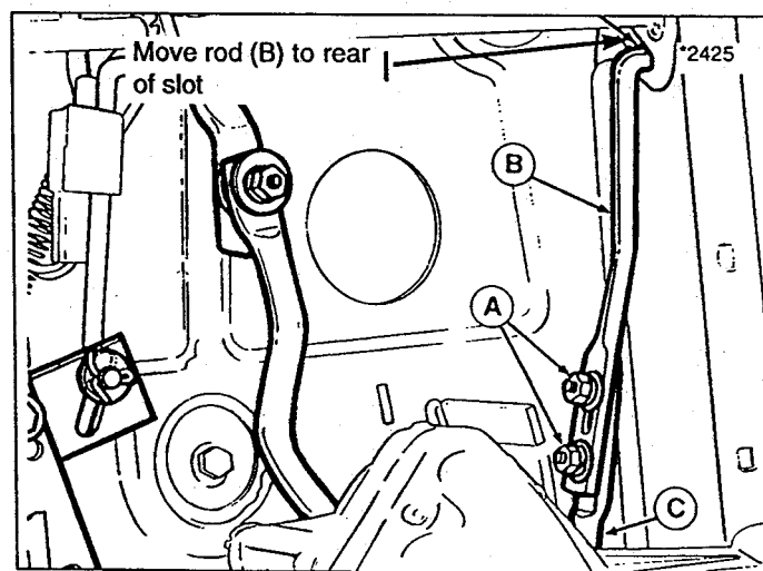
Figure 28. Return-To-Neutral Adjustment - Hydro Models
