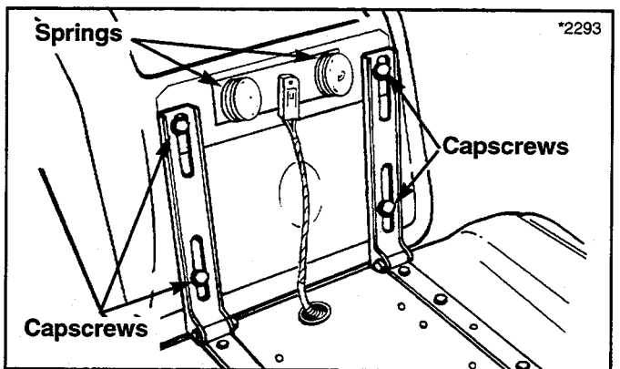
Figure 22 Seat Adjustment
