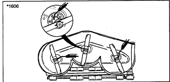
Figure 12. Mower Arbor
