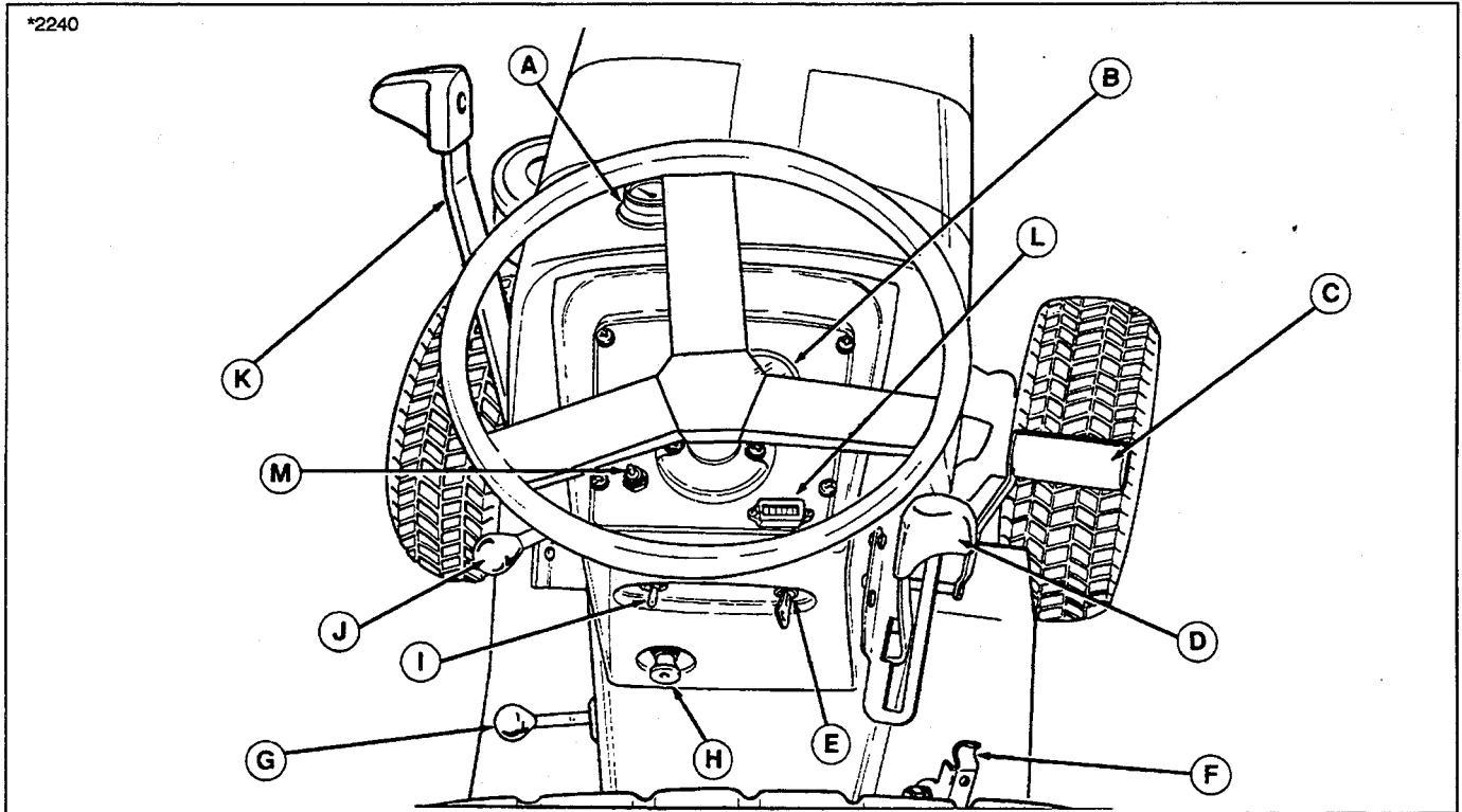
Figure 2. Tractor Controls
