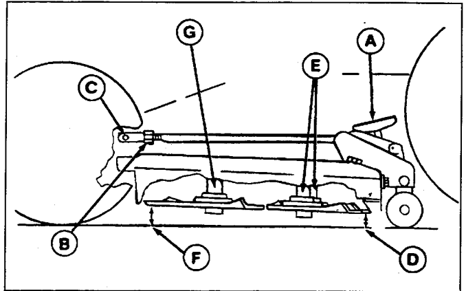
Figure 26. Mower Leveling
