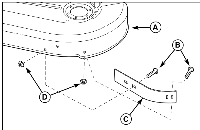
Figure 4. Baffle Removal
