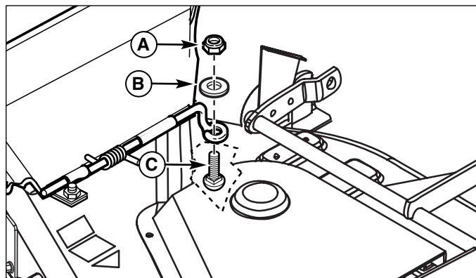
Figure 5. Carriage Bolt Removal
