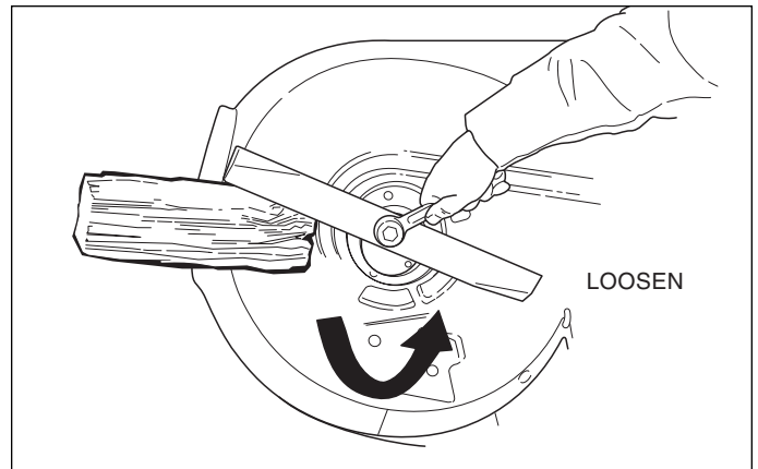
Figure 2. Blade Removal
