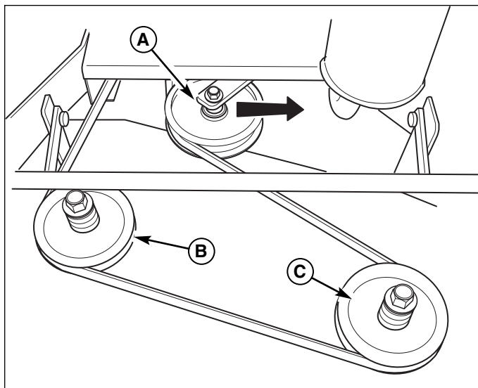
Figure 16. Mower Deck Drive Belt
