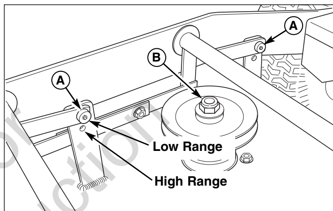
Figure 12. Pulley & Pivot Position
