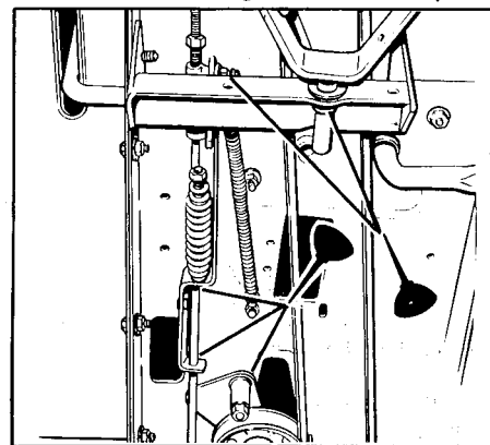
Figure 12. Clutch & Brake Rod Lubrication
