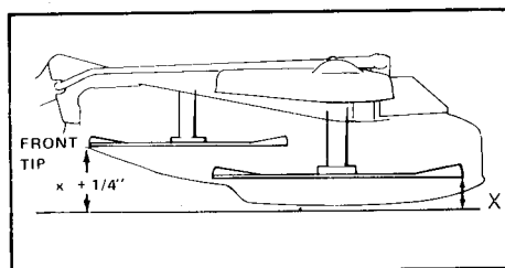
Figure 42. Levelling Mower - 42"
