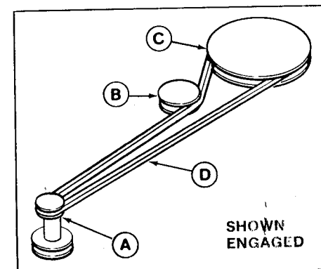
Figure 25. Tractor Belt Pattern
