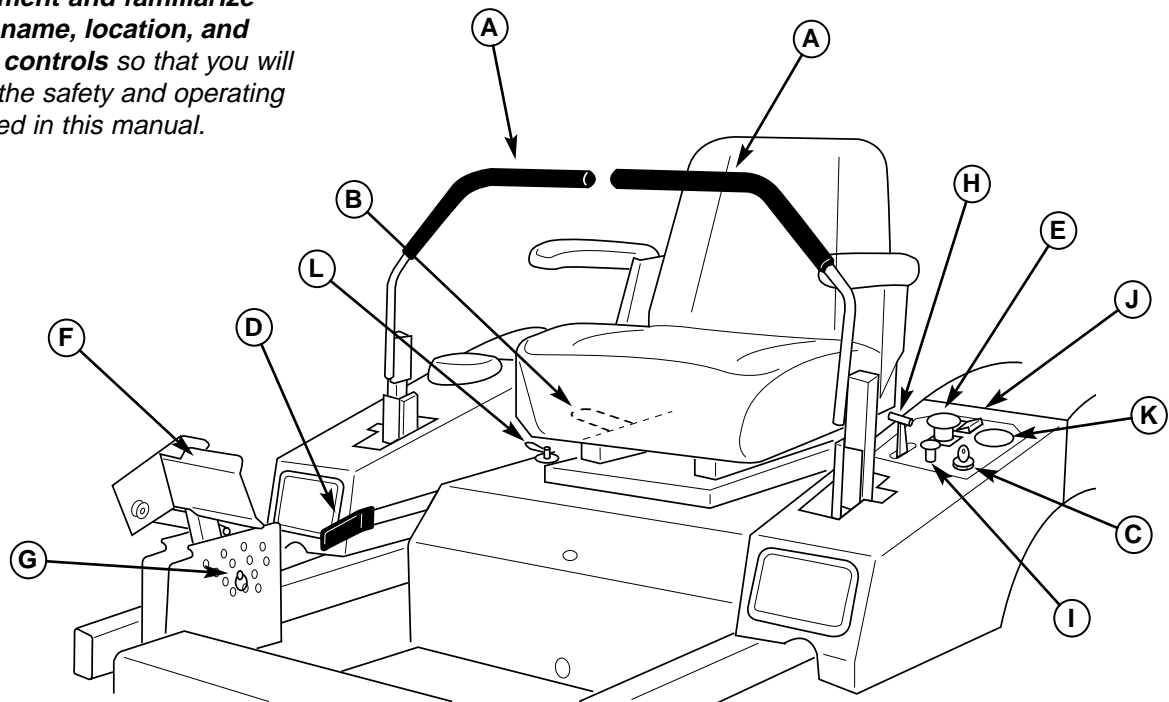
Figure 1. Control Locations
