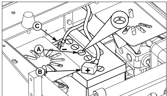
Figure 15. Battery Compartment
