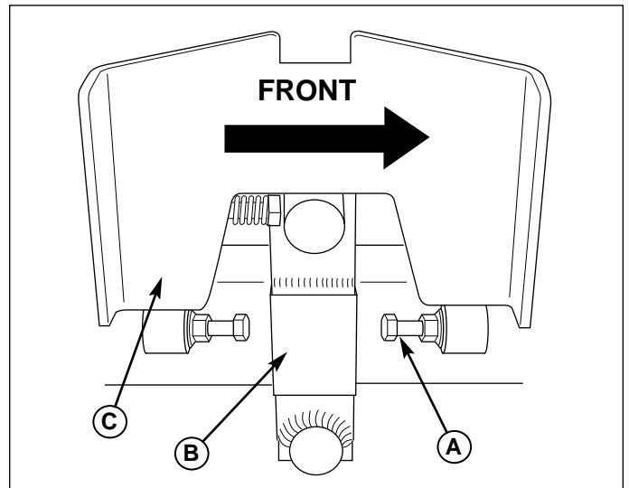
Figure 21. Top Speed Adjustment
