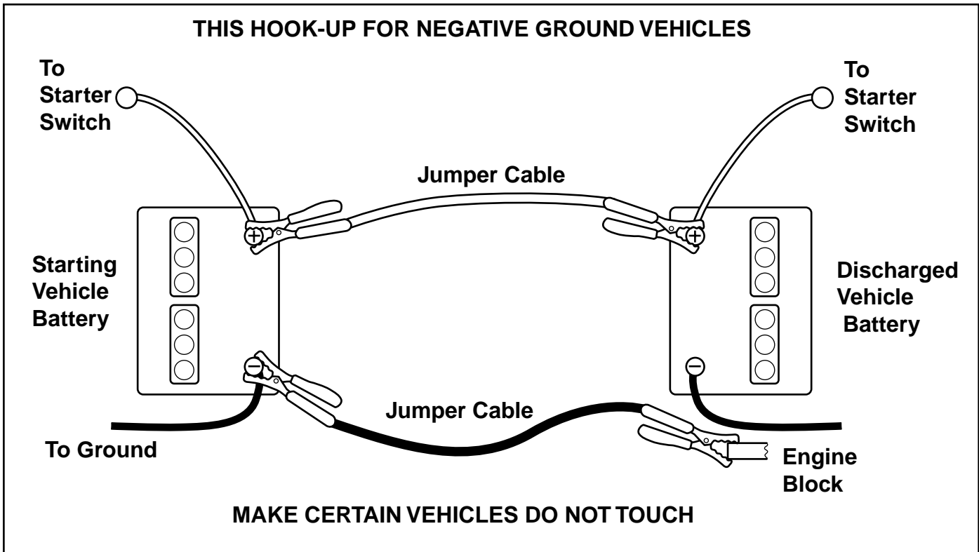
Figure 34. Jump Starting
