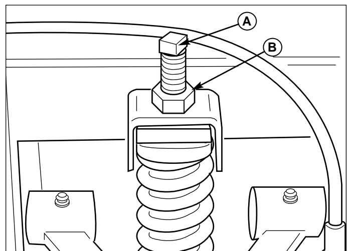
Figure 24. Suspension Height Adjustment
